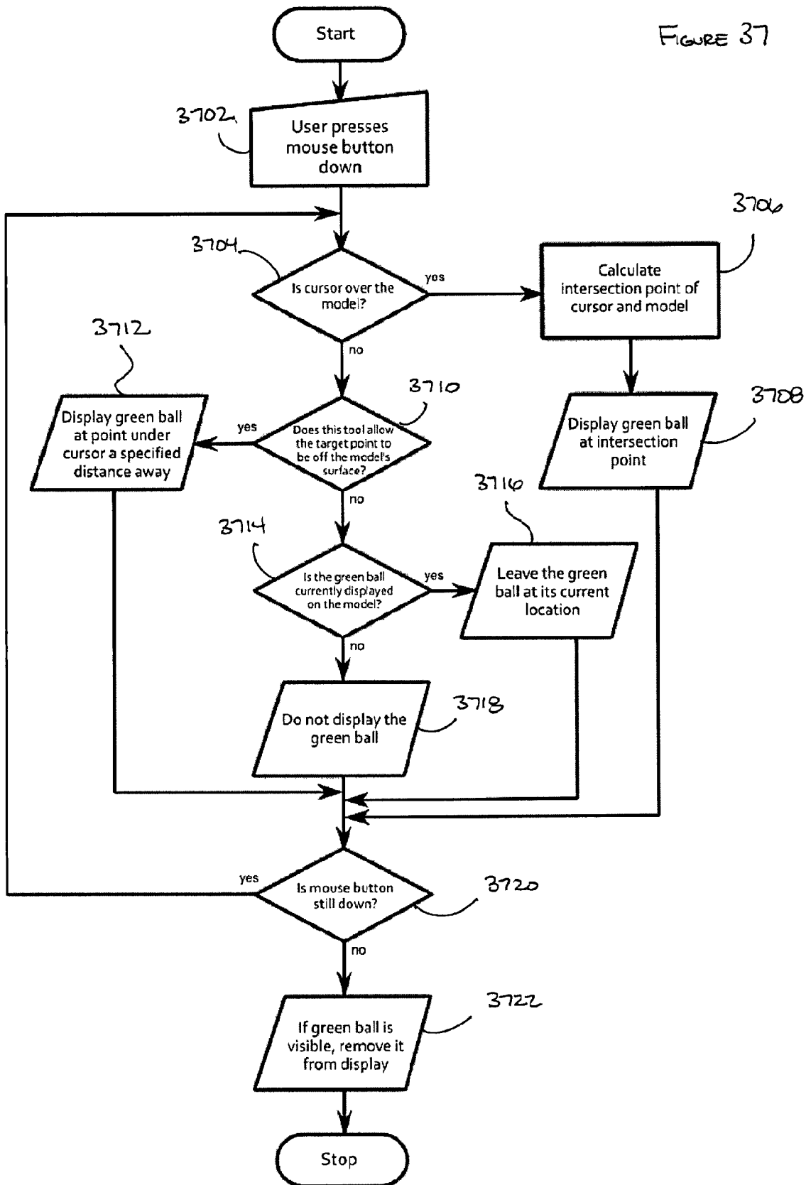
Flowchart of Green Ball Displaying
