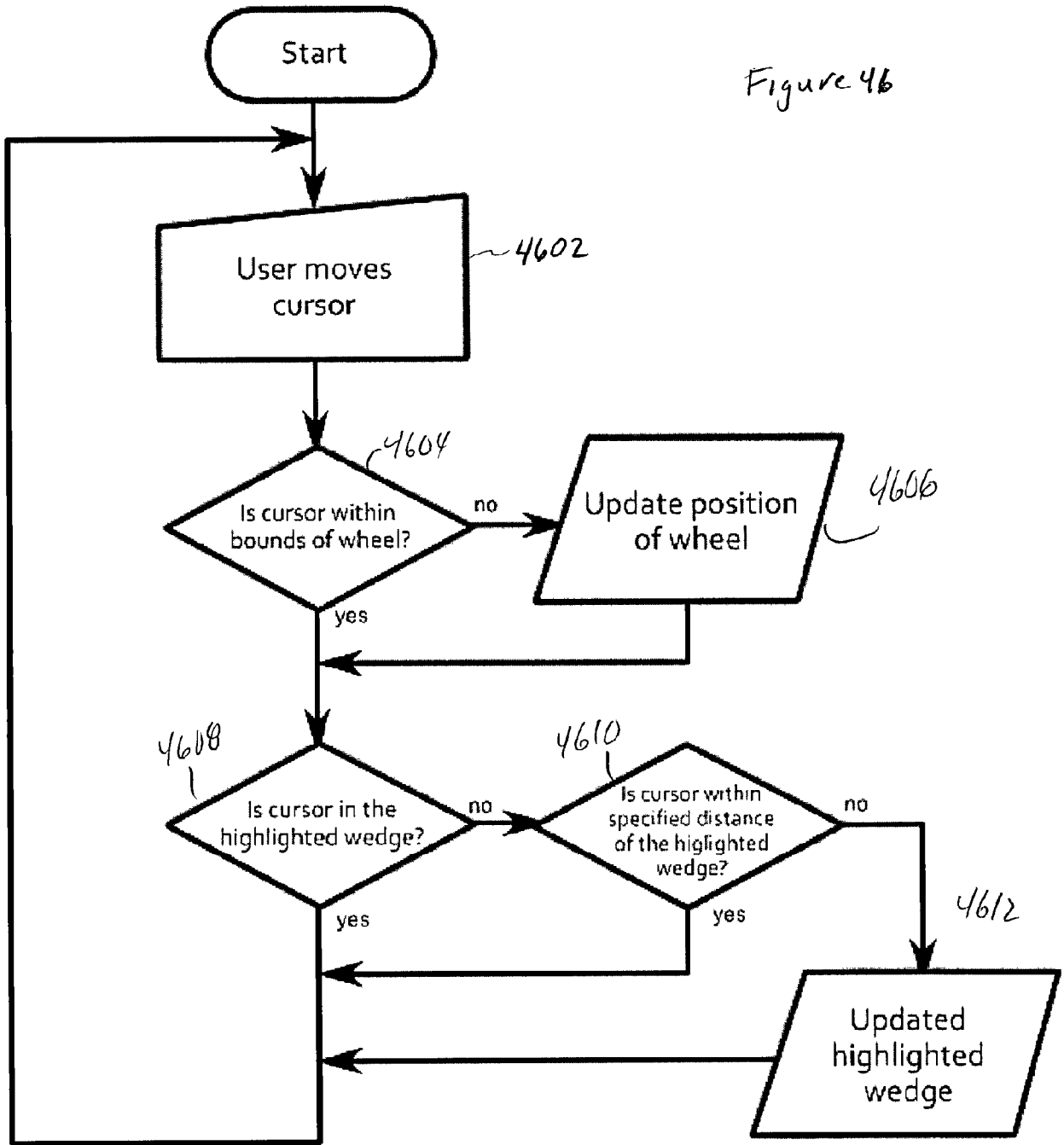
Flowchart of MiniWheel Wedge Activation
