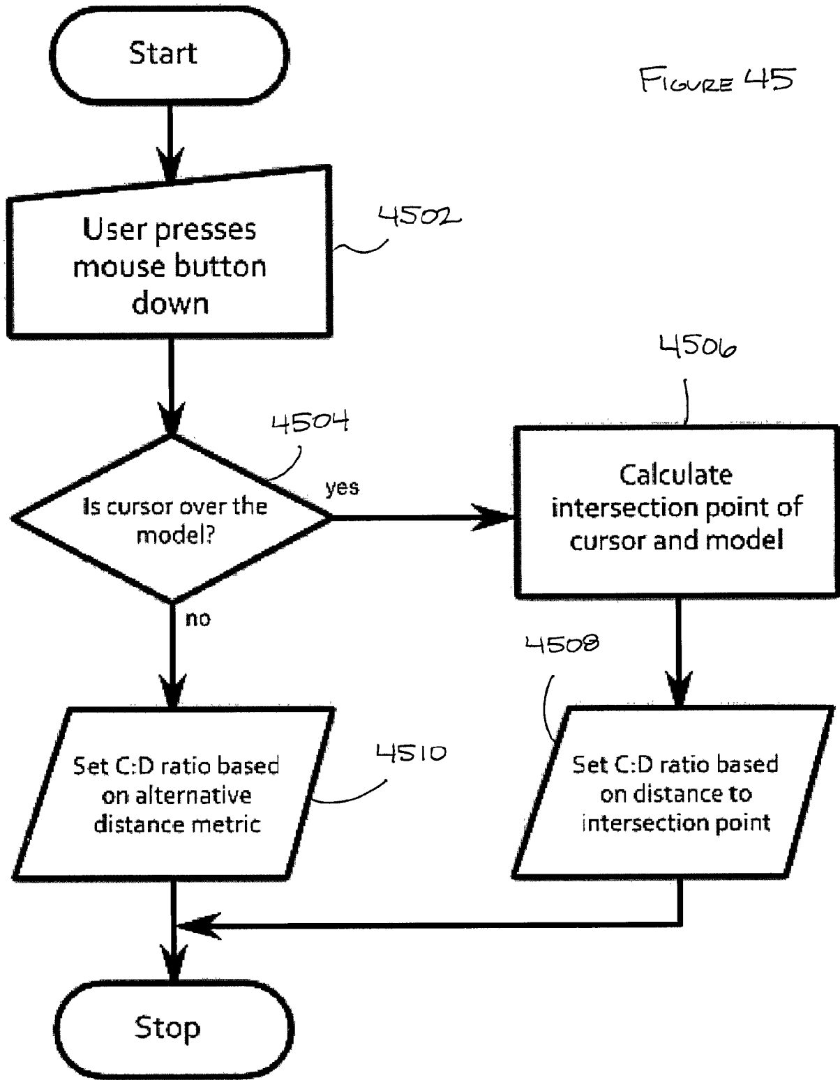
Flowchart of Pan Tool Initialization
