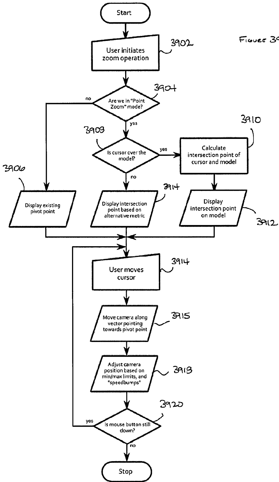
Flowchart of Zoom Tool
