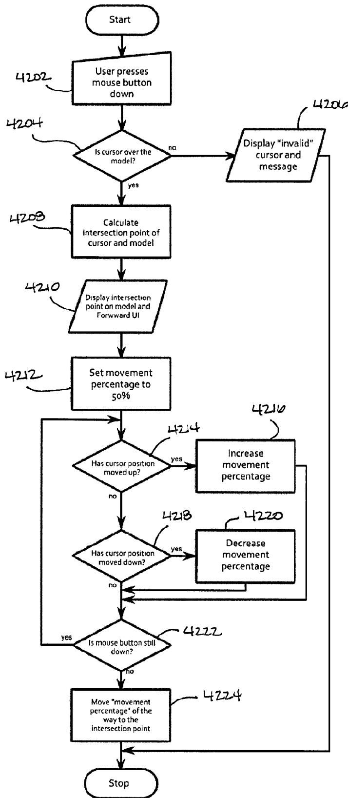
Flowchart of Forward Tool
