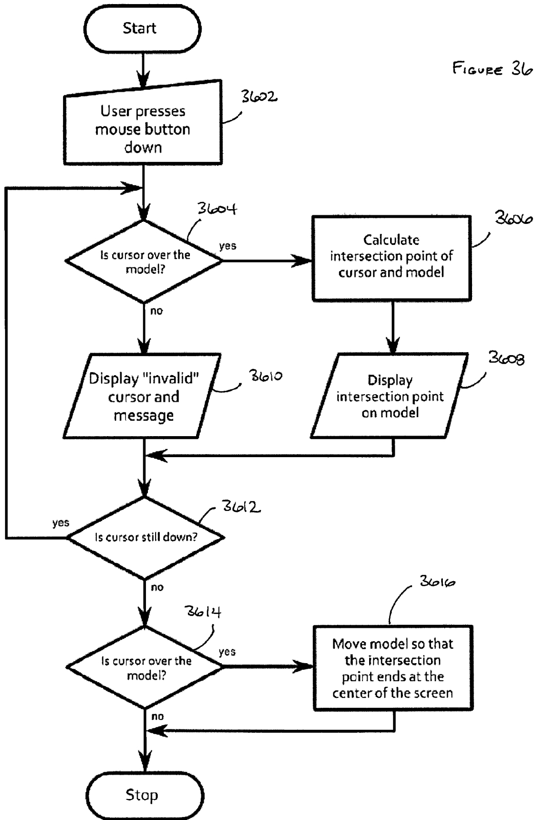
Flowchart of Center Tool
