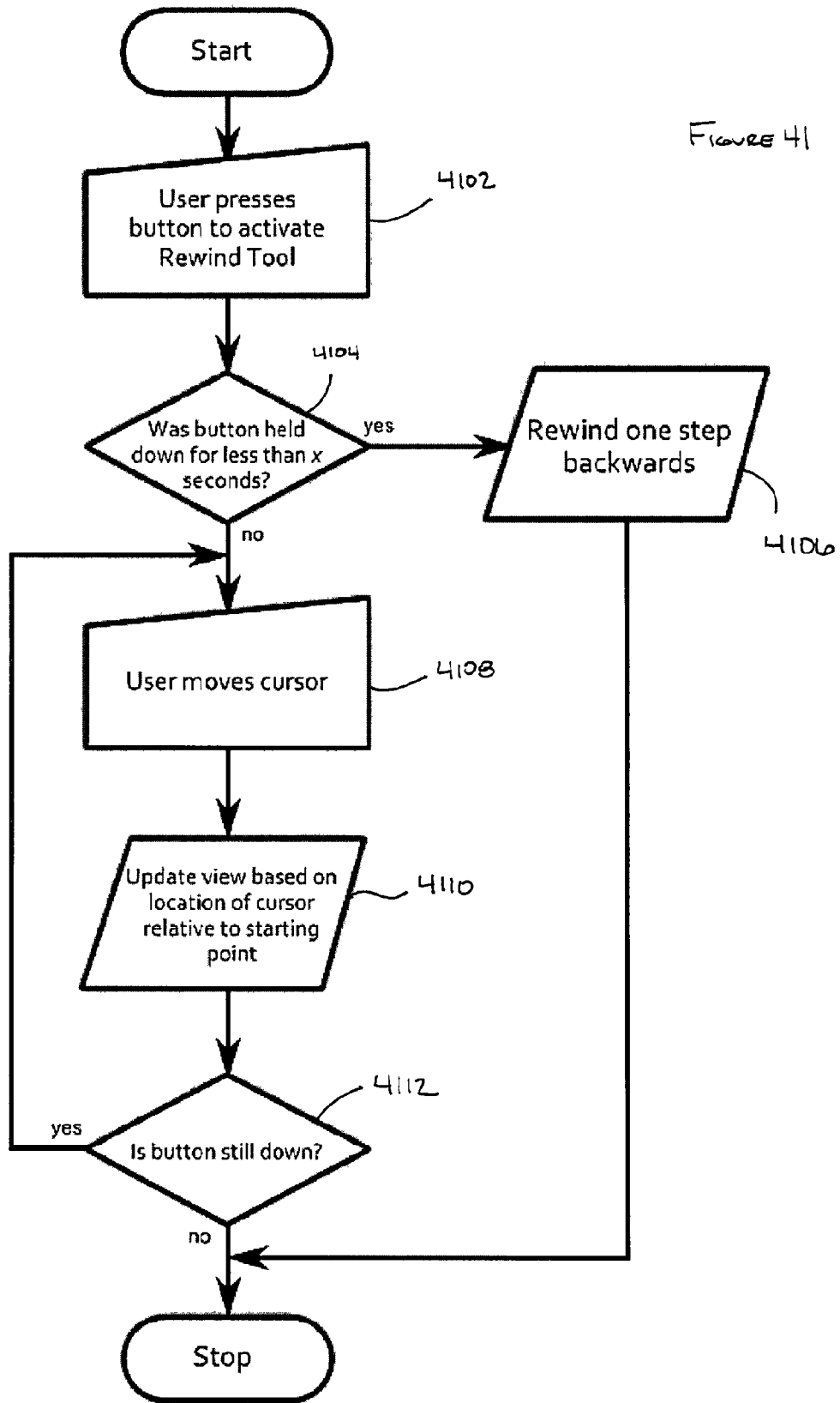
Flowchart of Rewind Tool Usage
