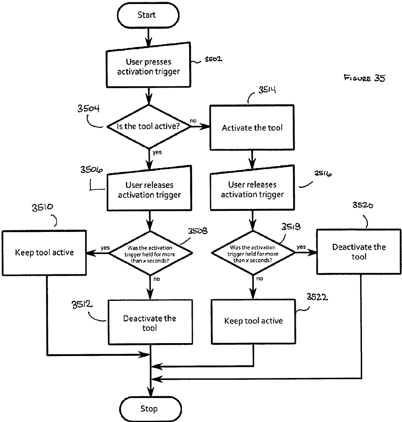
Flowchart of Tap vs. Hold Activation
