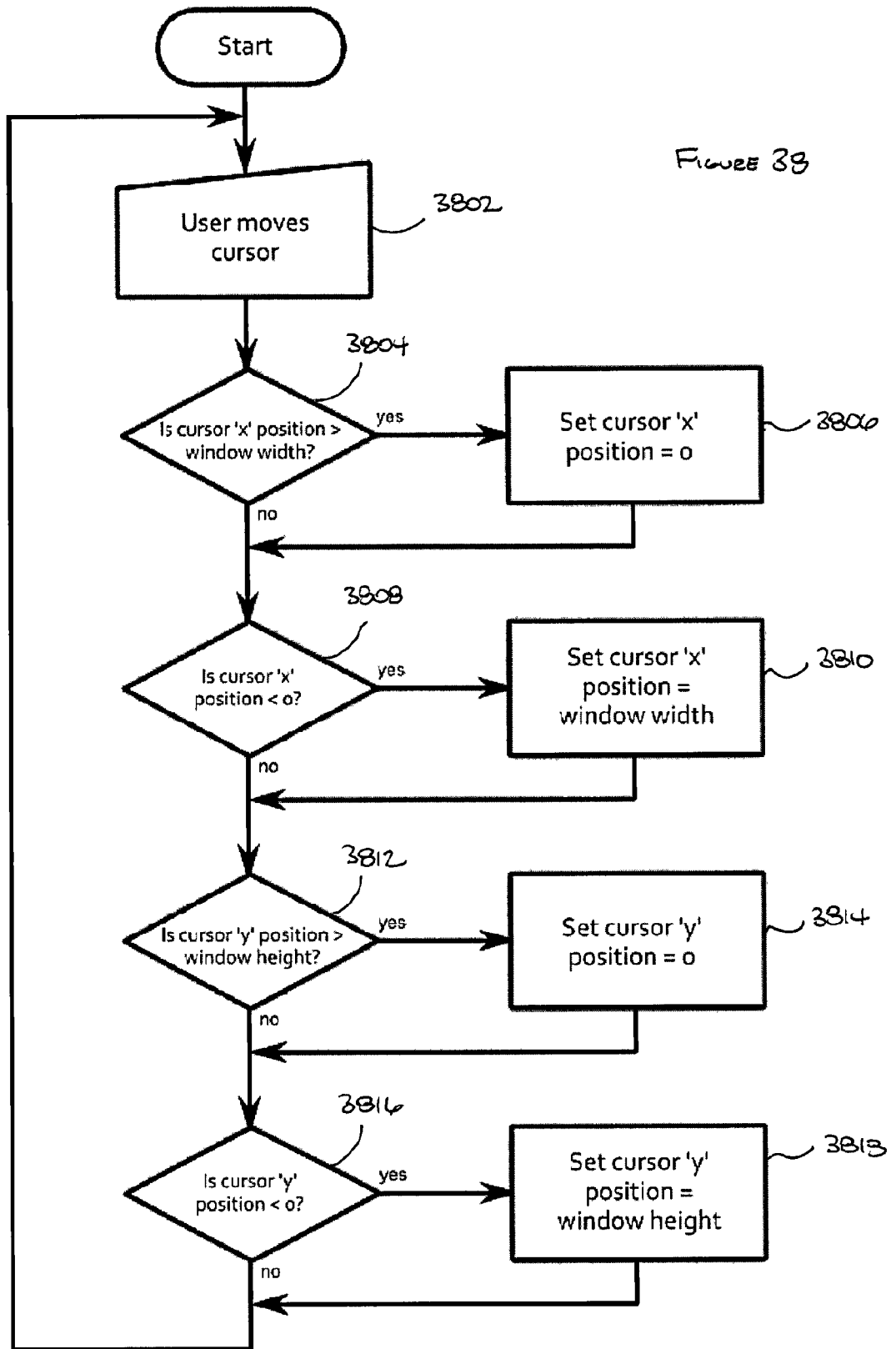
Flowchart of Window Cursor Wrapping
