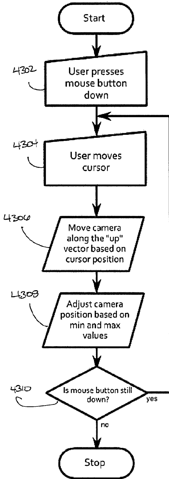
Flowchart of Up/Down Tool
