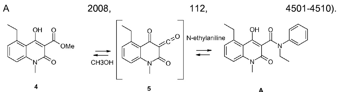
Scheme 2. An intermediate ketene 5 is involved in the equilibrium between 4 and A .
