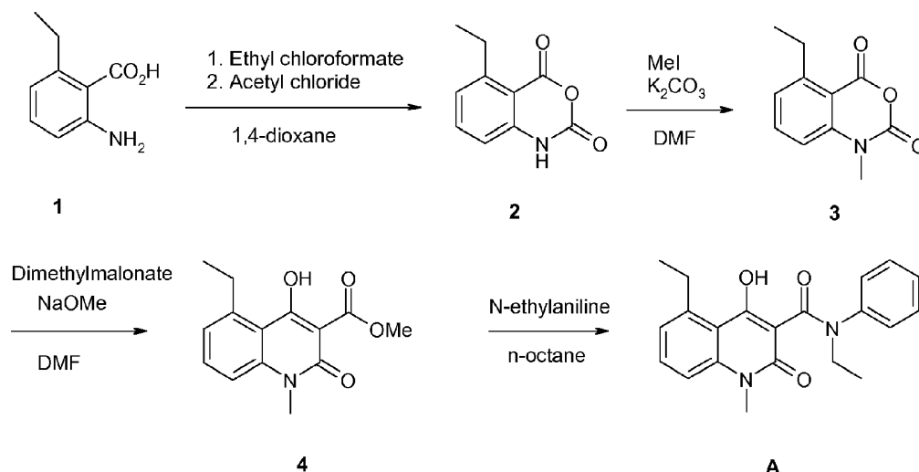
Scheme 1. The synthetic route to N-alkyl-N-phenyl-quinoline-3-carboxamides, exemplified with the synthesis of paquinimod ( A ) via the corresponding methyl ester 4 .
