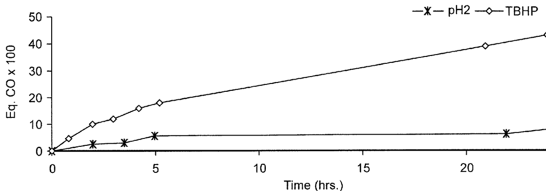
CO release by Trimethylacetaldehyde (compound 1)
