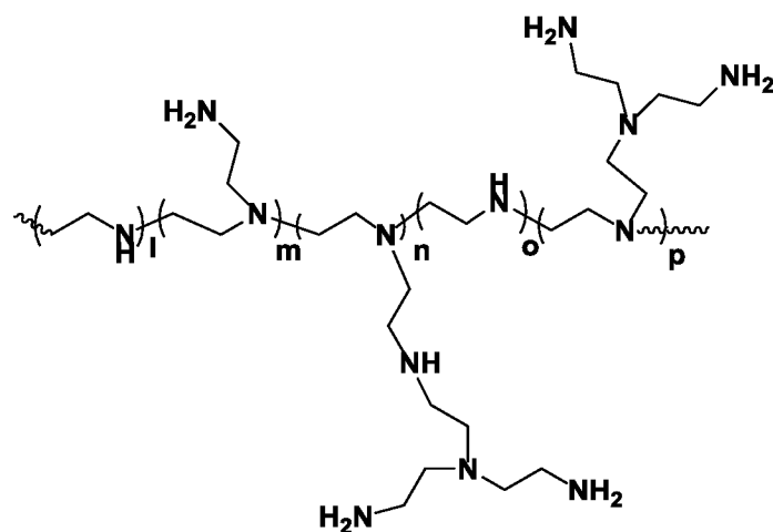
Branched Polyethyleimine
