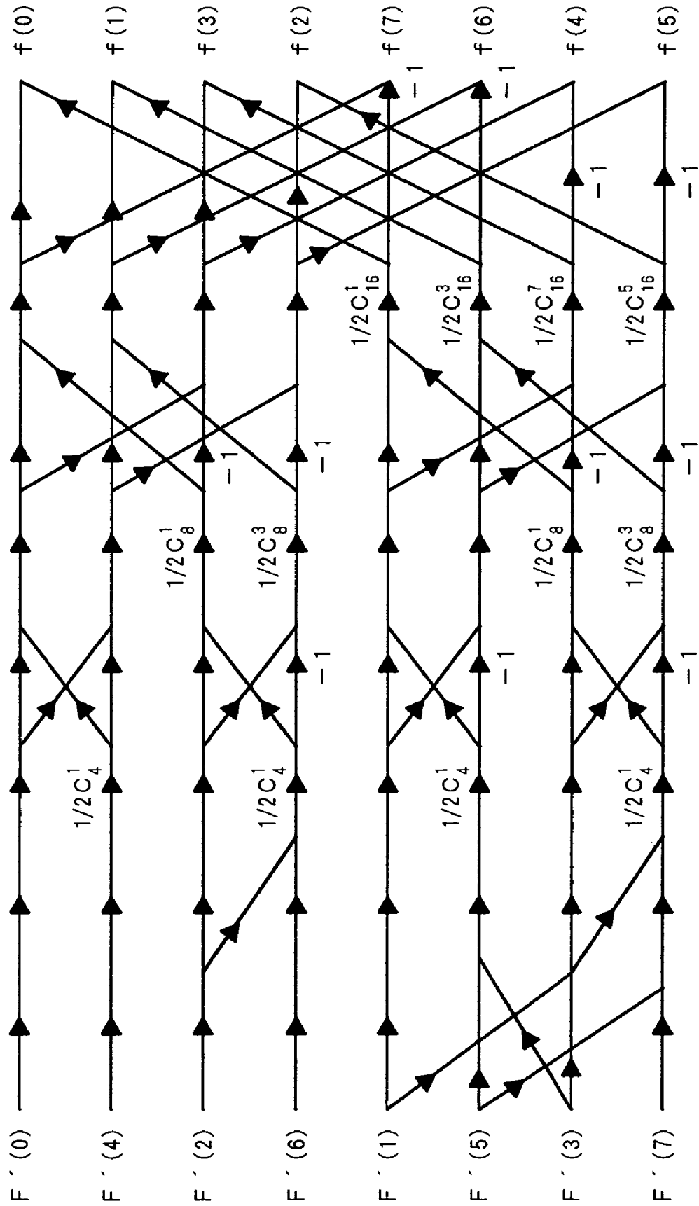
Fig. 15 PRIOR ART
