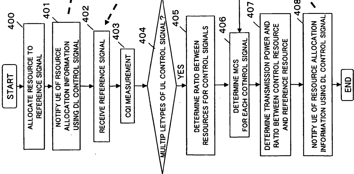
FIG.6A BASE STATION
