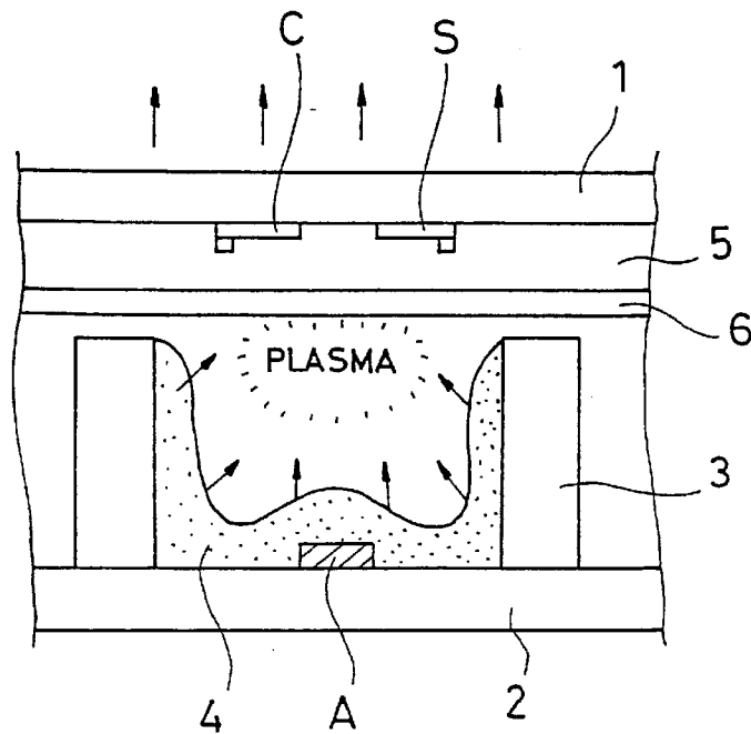
FIG. 3 (PRIOR ART)
