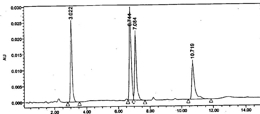
Figure 9a: HPLC profile – 7.5 hours at pH of 7.42
