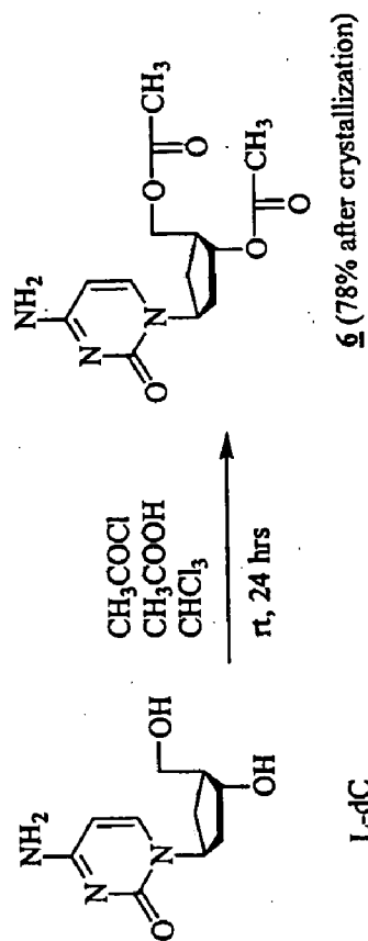
Figure 4: Synthesis of 3',5'-di-O-acetyl-2'-deoxy-β-L-cytidine
