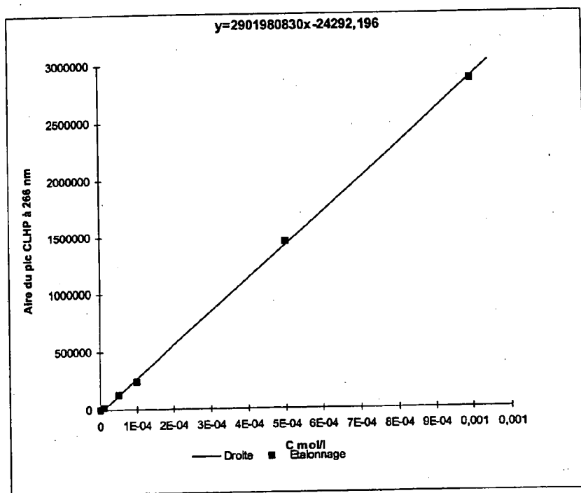
Figure 8b: Solubility Calibration Curve for the 3',5'-Divalinyl Ester of L-dC
