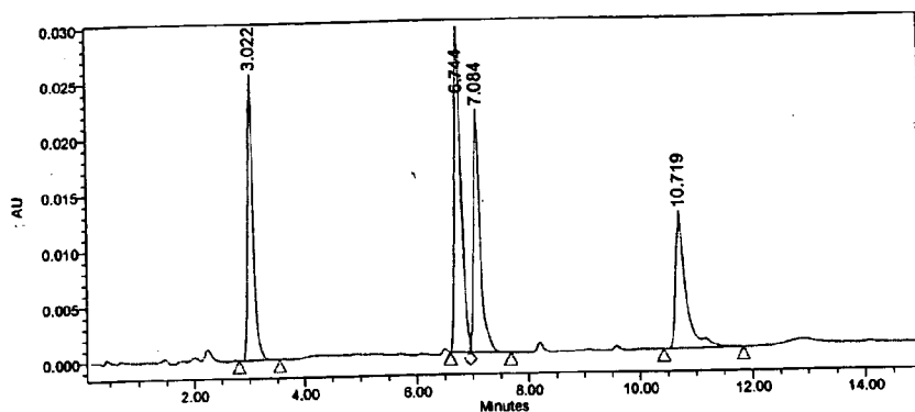
Figure 10a: HPLC profile – 5.33 hours at pH of 7.20
