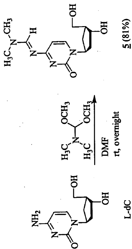
Figure 3: Synthesis of N' -[(dimethylamino)methylene]-2'-deoxy-β-L-cytidine
