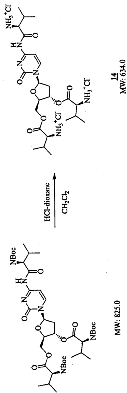
Figure 7: Synthesis of 3',5'- N' -tri-(L-valinyl)-L-2'-deoxycytidine
