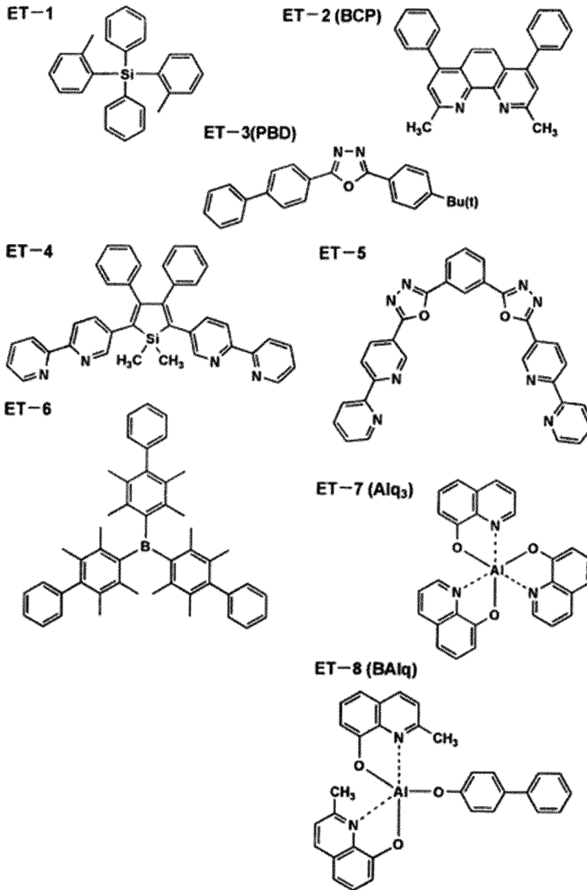
[Chem. 41]
