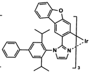
[Chem. 8]
