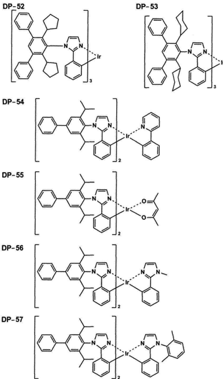
[Chem. 15]
