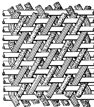
Triaxial Weave
