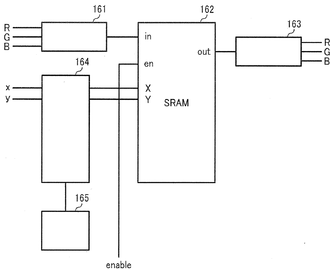
CONFIGURATION OF DISTORTION CORRECTION UNIT
