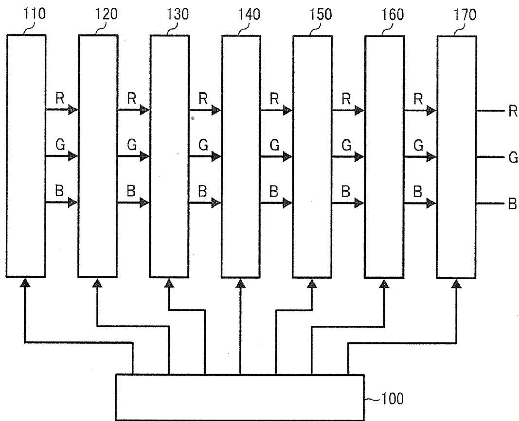
ENTIRE FUNCTION BLOCK DIAGRAM
