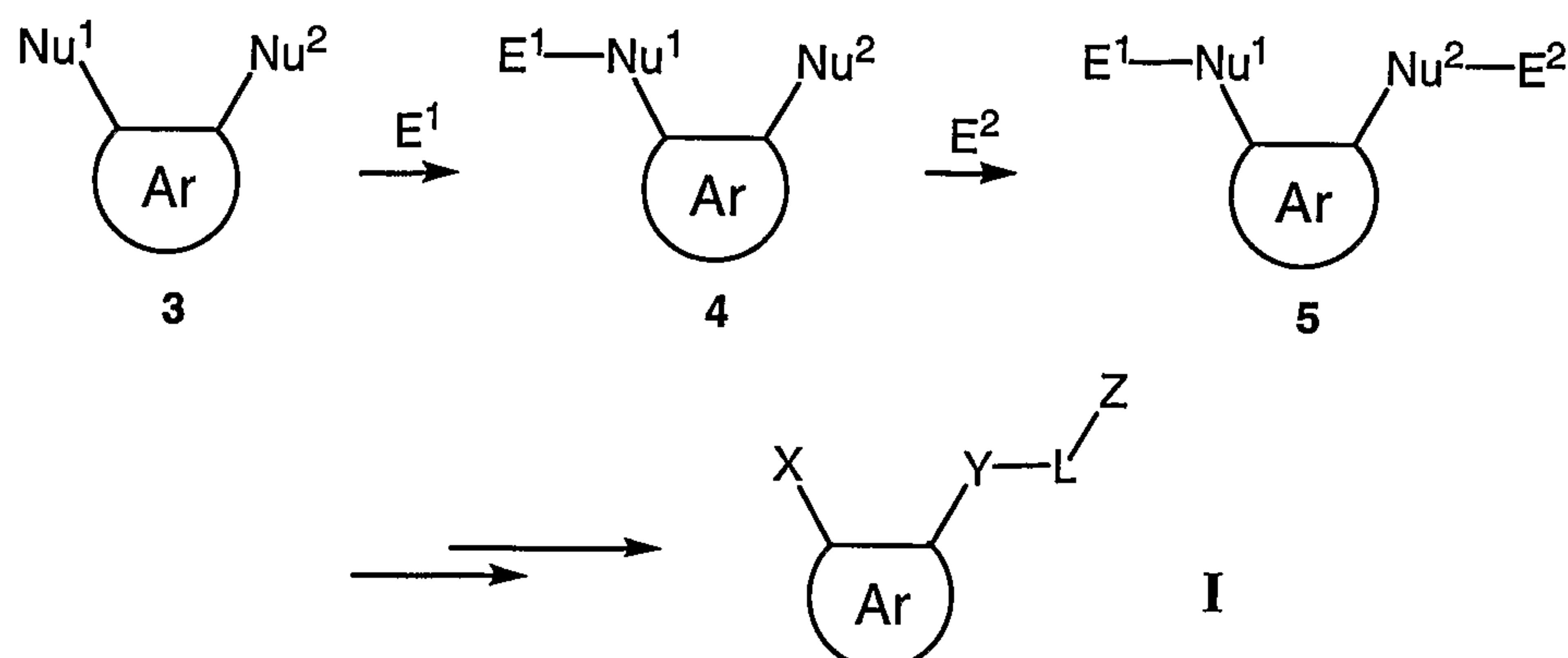
Scheme 2
