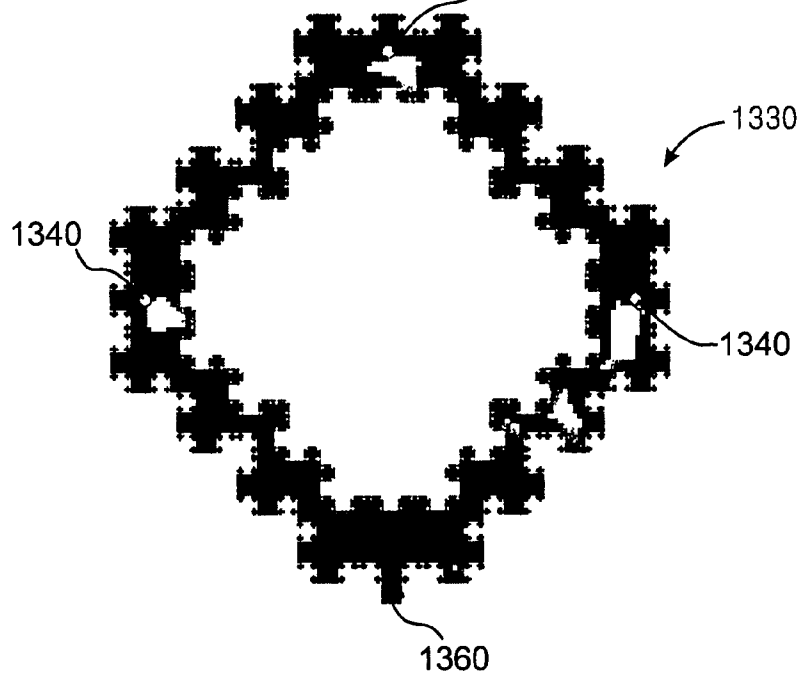
FIG. 14 CONDUCTING VIA 1340
