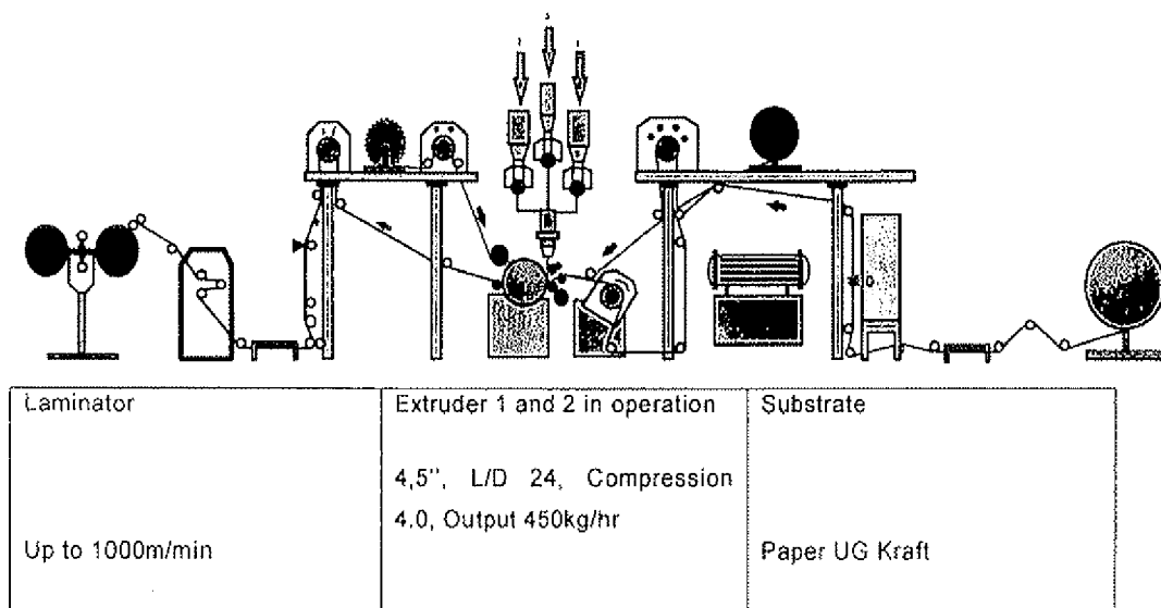
Figure 5: Extrusion Coating Setup
