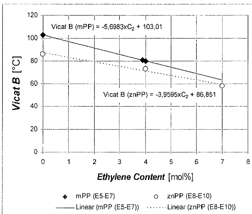
Figure 6: Vicat B of mPP and znPP as function of ethylene content for homo- and copolymers
