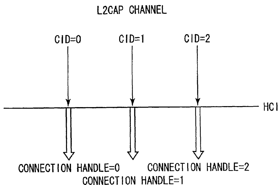
FIG. 6 CORRESPONDENCE 1 BETWEEN L2CAP CHANNEL AND CONNECTION HANDLE
