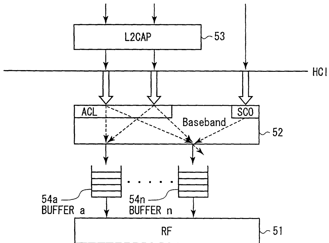
FIG. 12 PROVIDING A BUFFER FOR EACH DIFFERENT SERVICE CLASS (INCLUDING SCO LINK)
