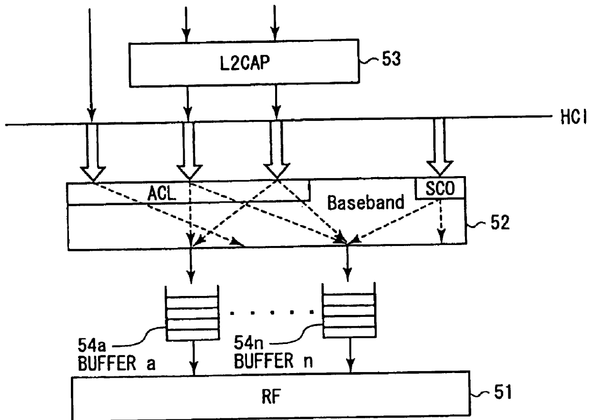
FIG. 14 XAMPLE 2 WHERE THERE IS A SERVICE USED BY THE OTHER ACL LINK
