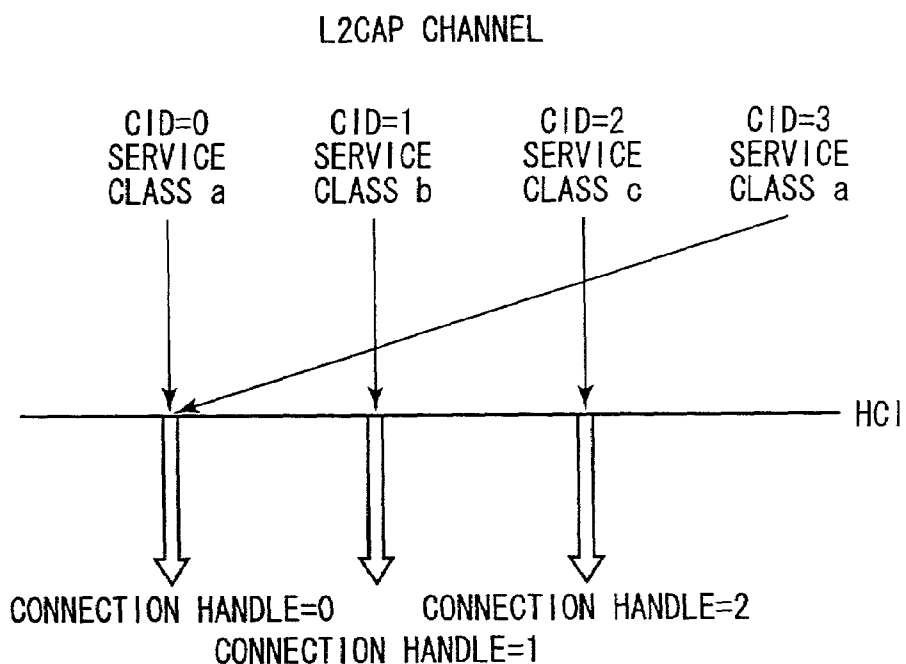
FIG. 7 CORRESPONDENCE 2 BETWEEN L2CAP CHANNEL AND CONNECTION HANDLE
