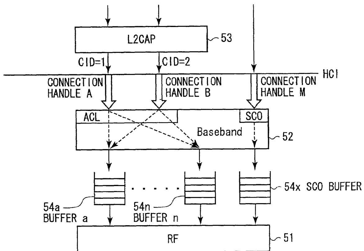
FIG. 5 PROVIDING A BUFFER FOR EVERY DIFFERENT SERVICE CLASS (INDEPENDENT FROM SCO LINK)
