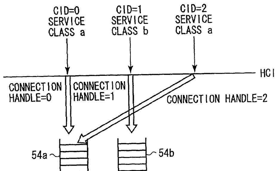
FIG. 8 CORRESPONDENCE 1 BETWEEN CONNECTION HANDLE AND BUFFER
