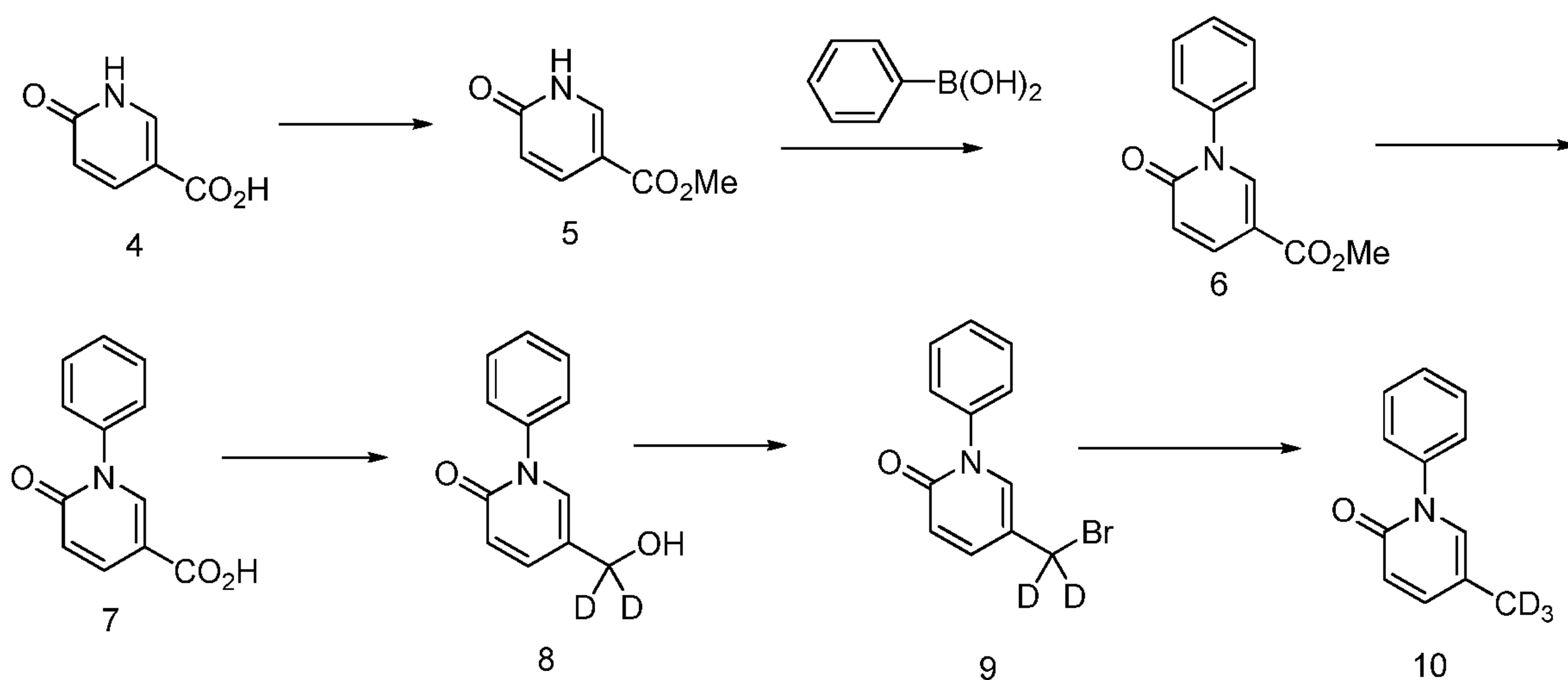
Scheme 2
