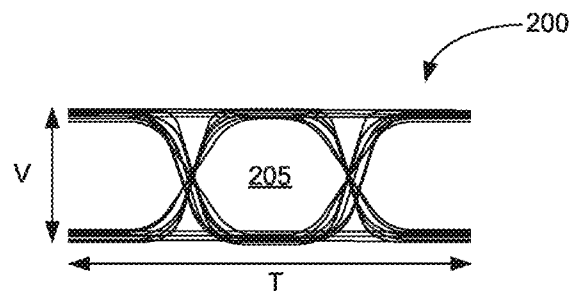
FIG. 2 (PRIOR ART)
