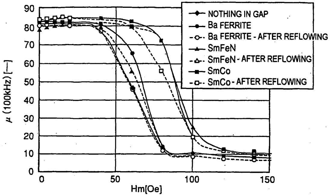
DC SUPERPOSED CHARACTERISTIC
