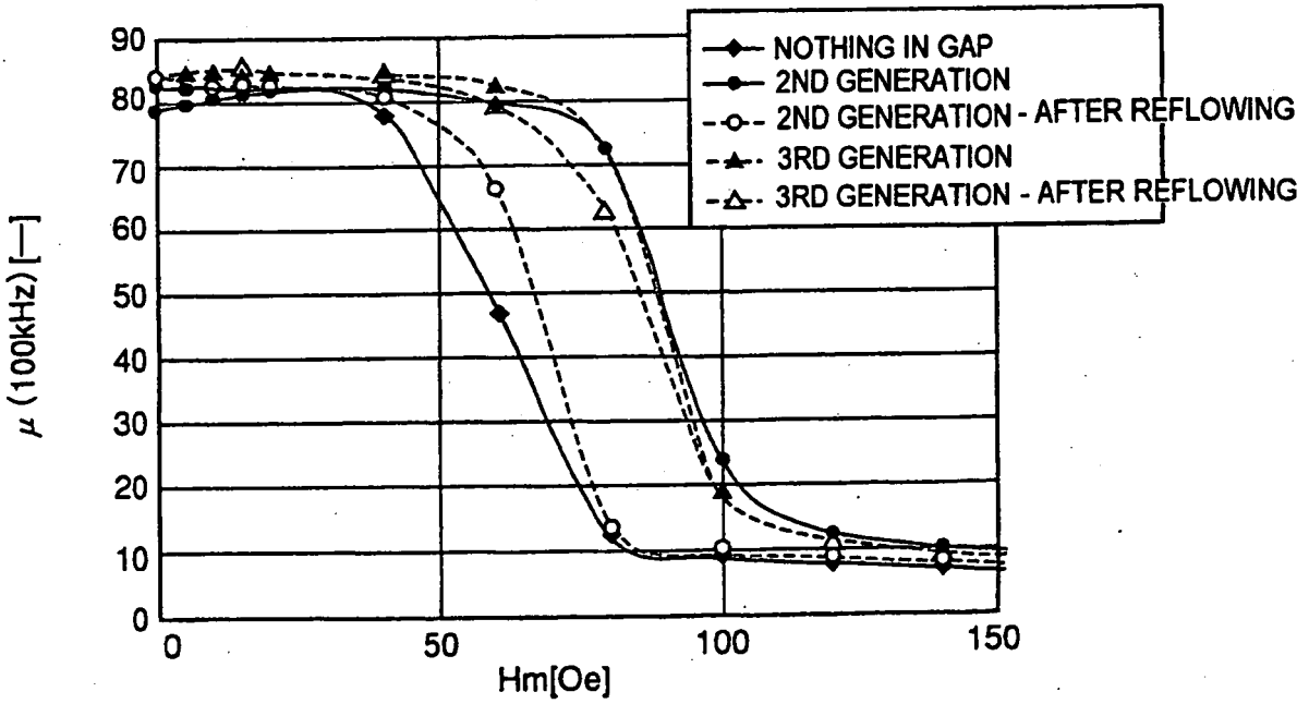
DC SUPERPOSED CHARACTERISTIC
