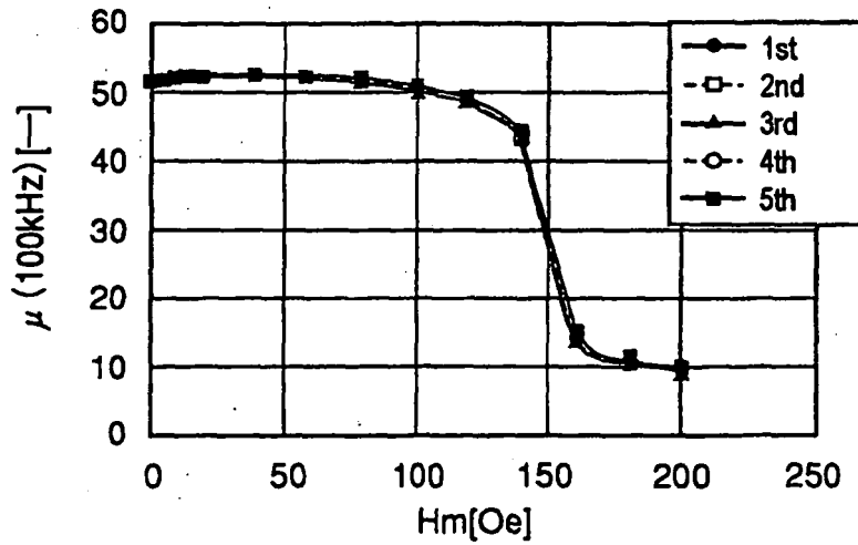
DC SUPERPOSED CHARACTERISTIC (Hc:10kOe)
