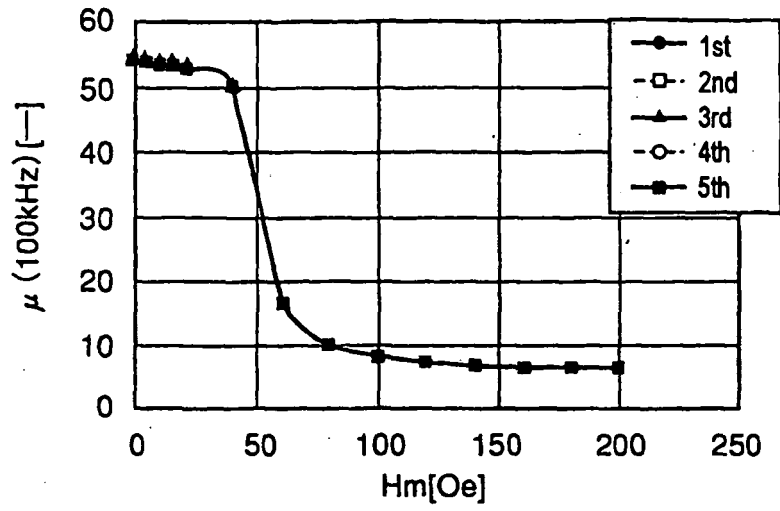
DC SUPERPOSED CHARACTERISTIC (GaP)
