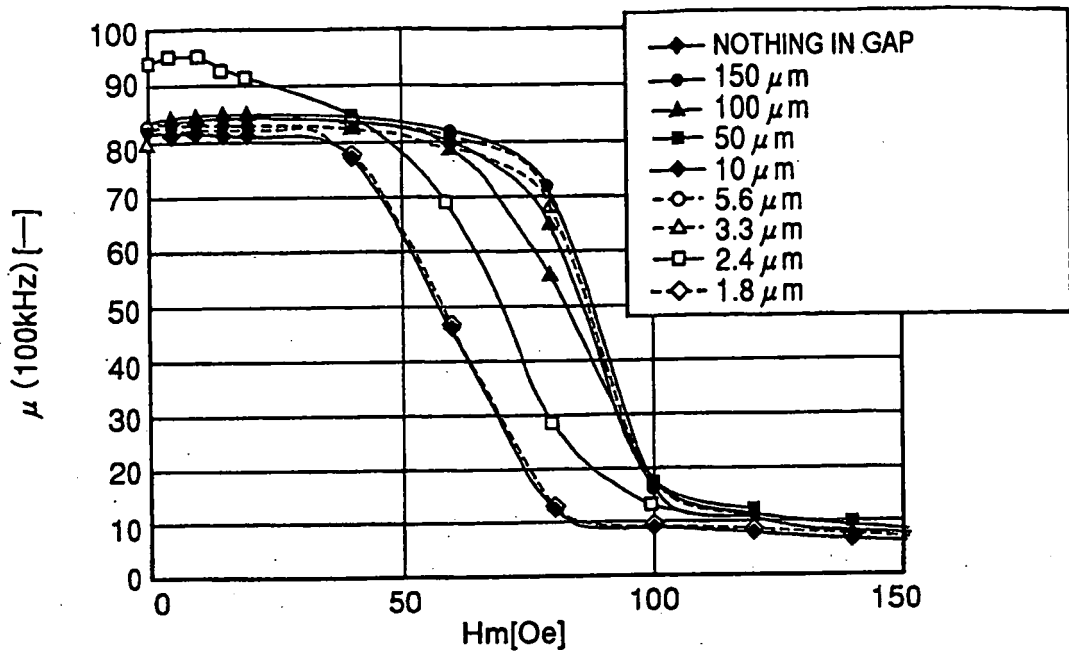
DC SUPERPOSED CHARACTERISTIC
