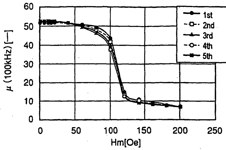
DC SUPERPOSED CHARACTERISTIC (Hc:5.0kOe)
