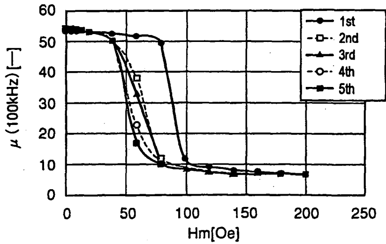
DC SUPERPOSED CHARACTERISTIC (Hc:4.0kOe)
