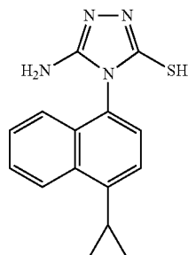
5-Amino-4-(1-cyclopropylnaphthalen-4-yl)- 4H-1,2,4-triazole-3-thiol
