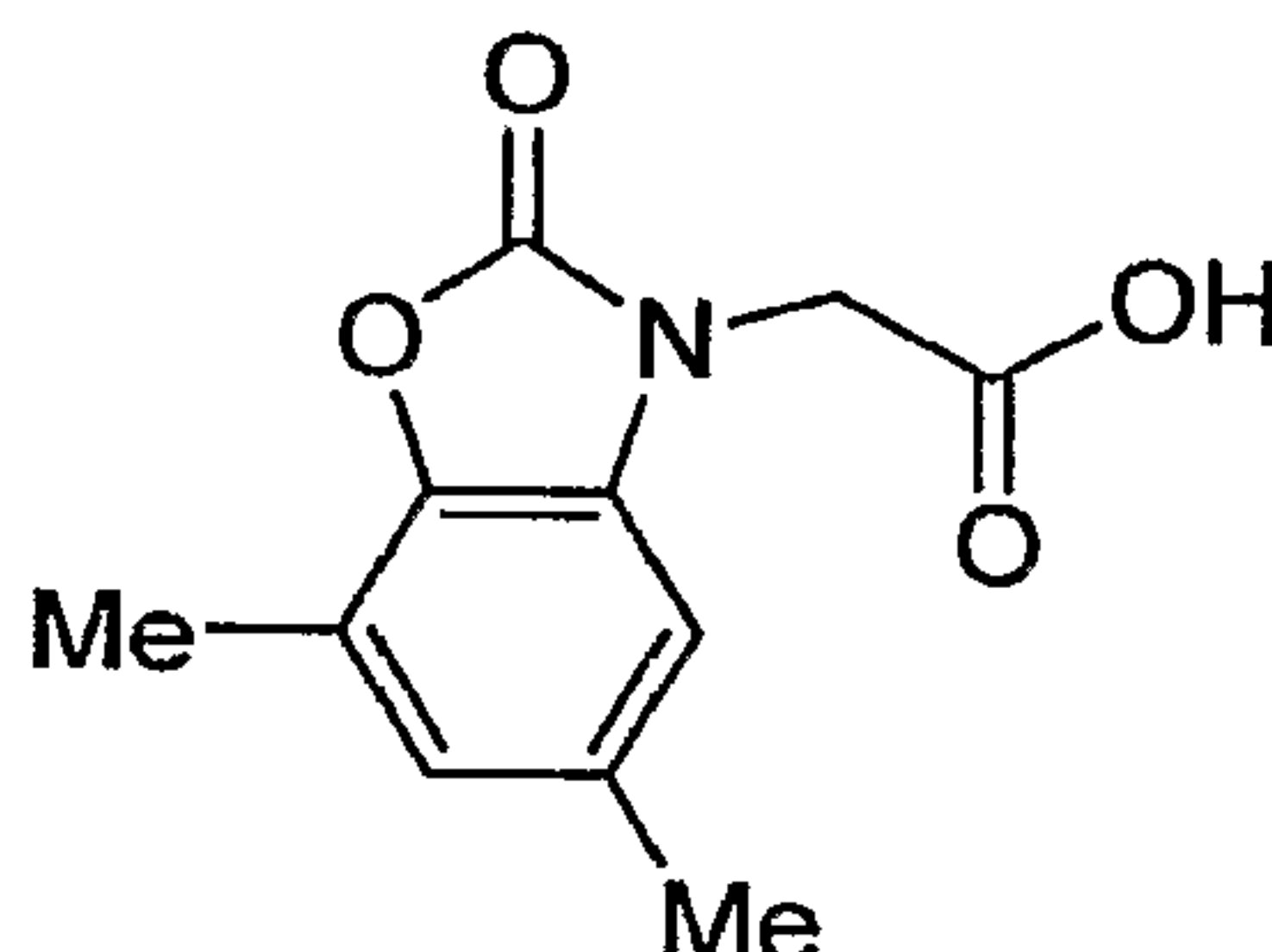
(5,7-Dimethyl-2-oxo-1,3-benzoxazol-3(2H)-yl)acetic acid
