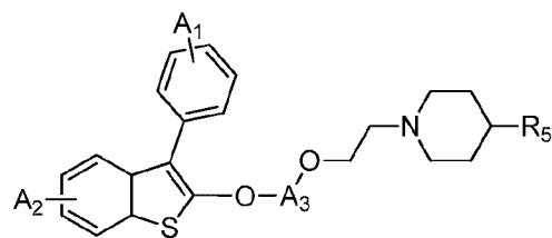
(Ia-ii)
