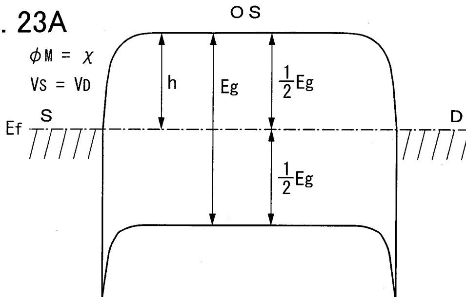
Energy Band Diagram in A-A' Cross Section
