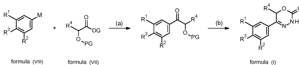
Scheme 9
