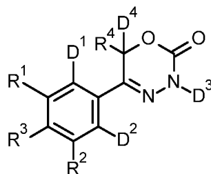
formula (Ia)
