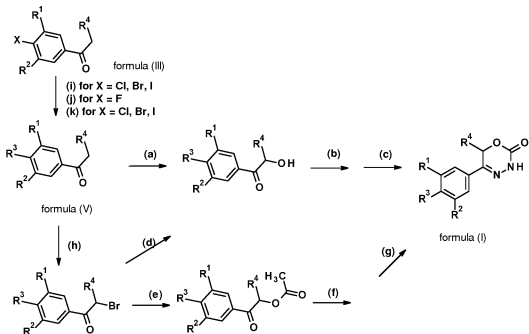
Scheme 4
