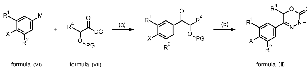
Scheme 8
