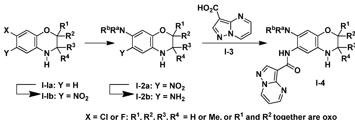
SCHEME I
