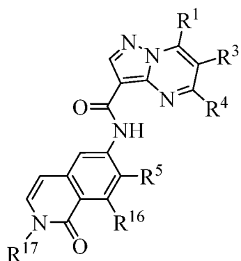
Formula VII;
