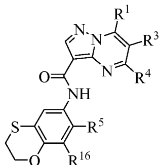
Formula V;
