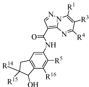
Formula III;
