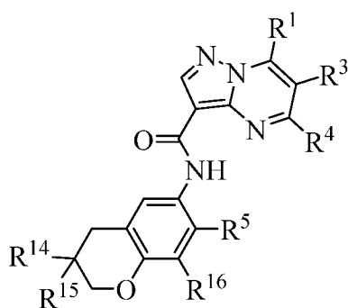
Formula VIII;
