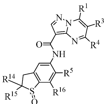
Formula VI;
