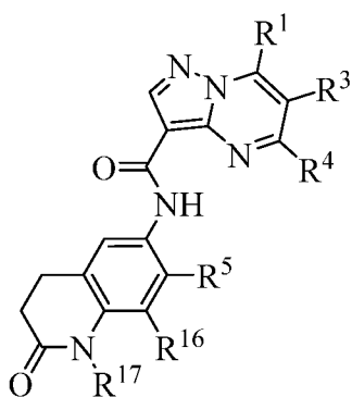
Formula IV;
