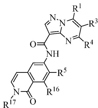
Formula VII;
