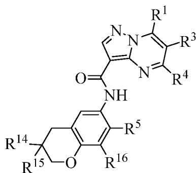
Formula VIII;
