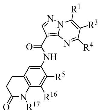
Formula IV;
