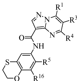
Formula V;
