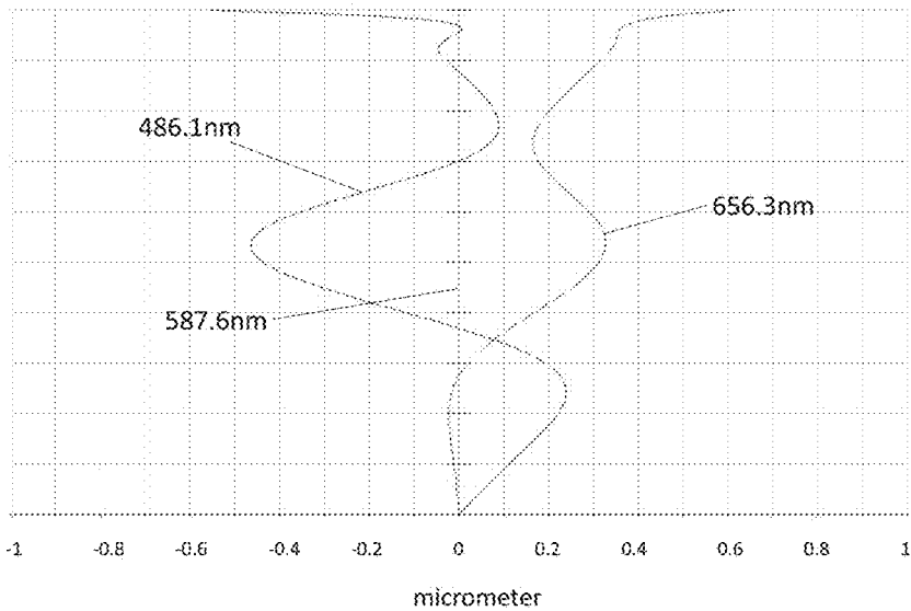
Lateral color
