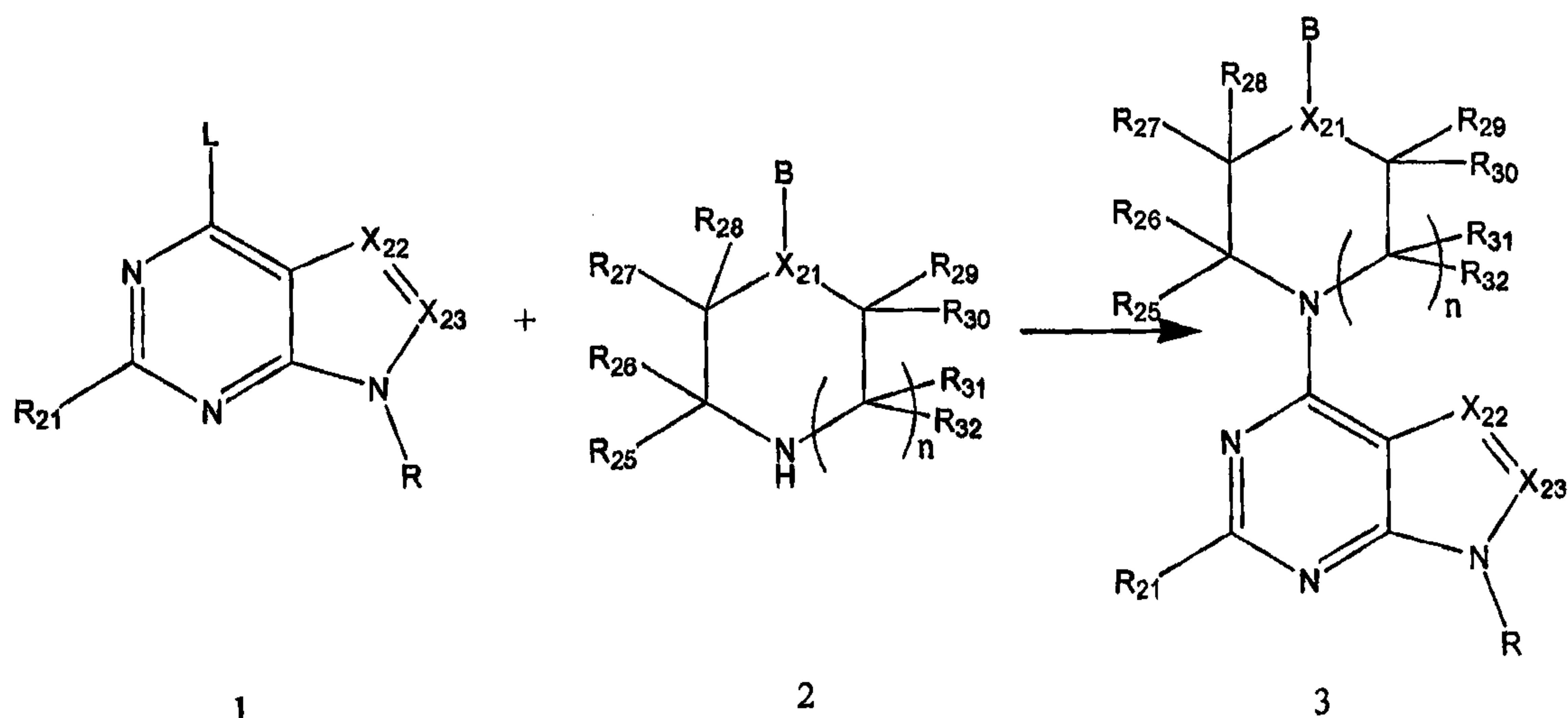
Scheme 1
