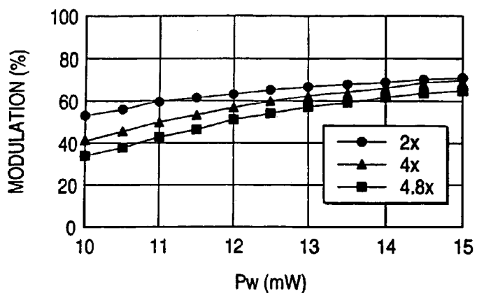
RECORDING POWER DEPENDENCY OF MODULATION
