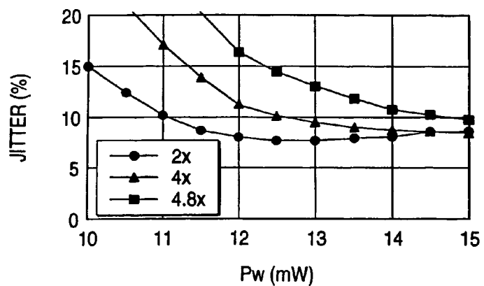
RECORDING POWER DEPENDENCY OF EDGE-TO-CLOCK JITTER
