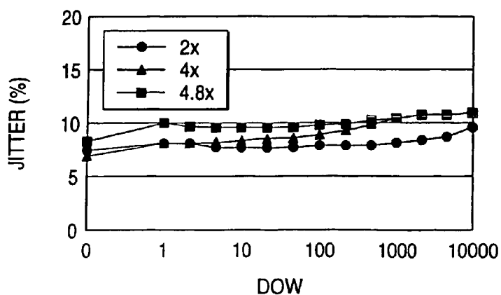
OVERWRITE CYCLE DEPENDENCY OF EDGE-TO-CLOCK JITTER
