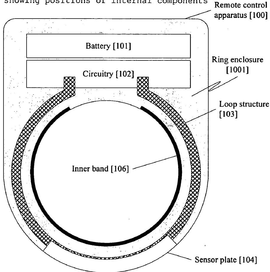
Cross-section of remote control apparatus showing positions of internal components
