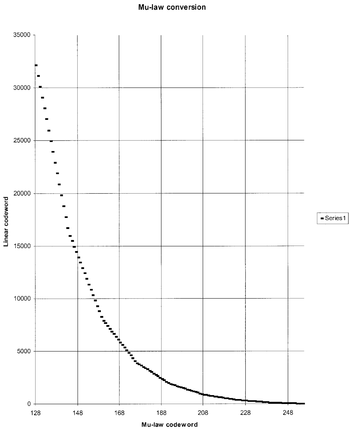
Fig. 3 Prior Art
