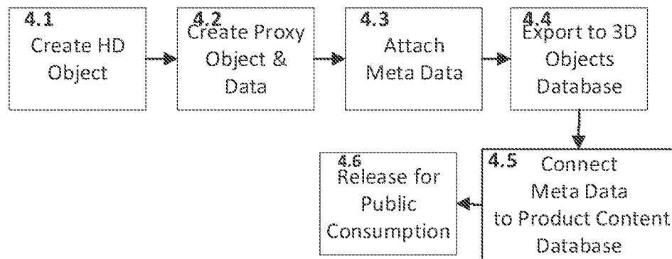
Figure 4: Creating New 3D Objects
