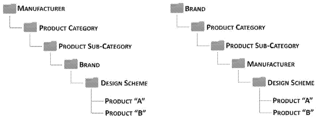
Figure 14: Example of Dynamically Managing Menu Structure for 3D Object and Product Data
