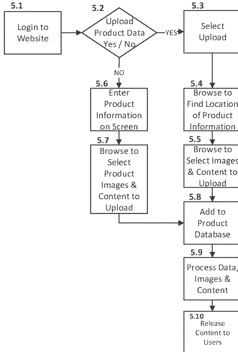
Figure 5: Adding Product Data to Product Database
