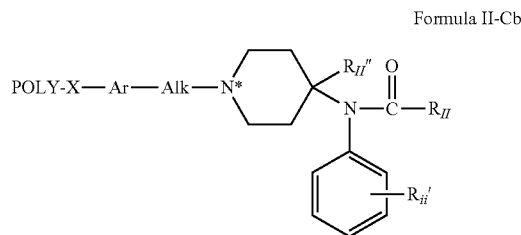
Formula II-Cb
