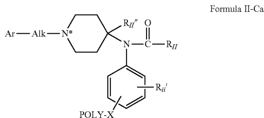
Formula II-Ca
