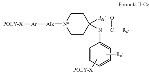
Formula II-Cc
