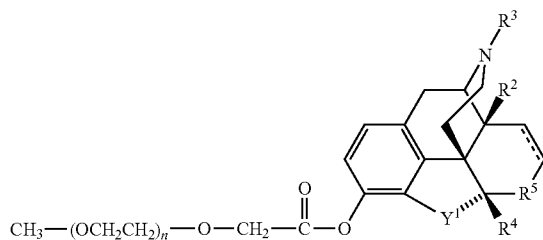
Formula I-Cd
