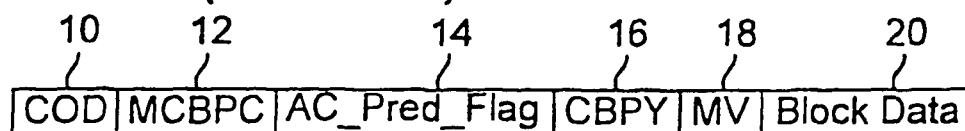
FIG. 1 (Prior Art)
