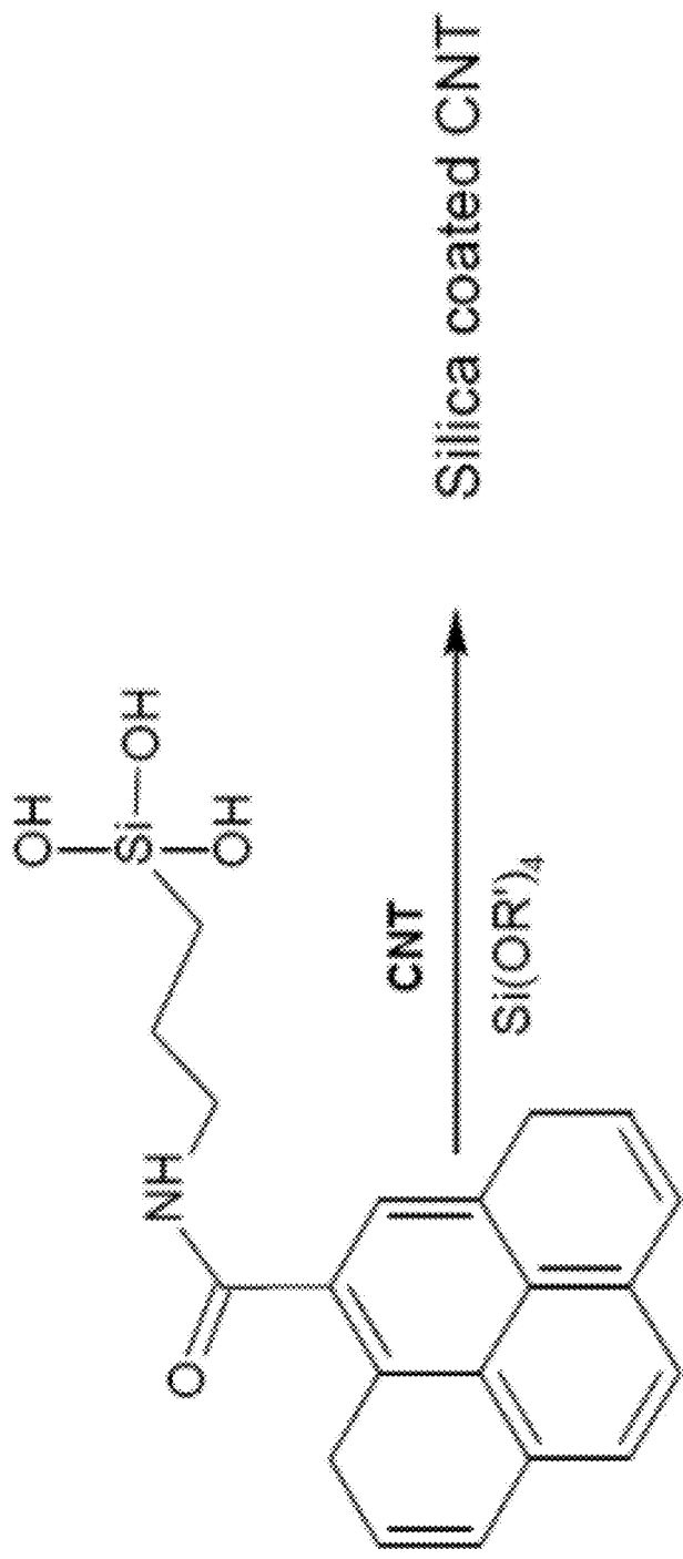
Pyrene derivative
