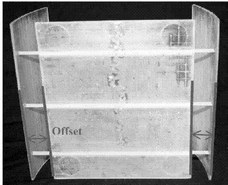
Figure 26: Offset Dimension
