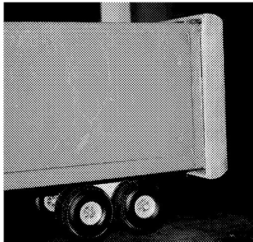
Airfoil Vane Concept on the Model
