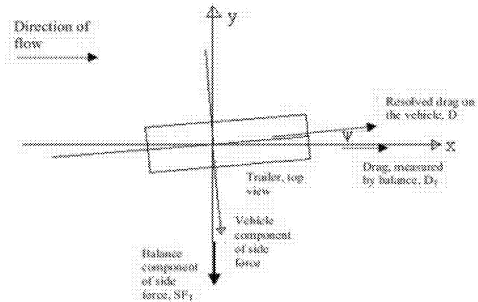
Figure 14: Side and Drag Force Schematic
