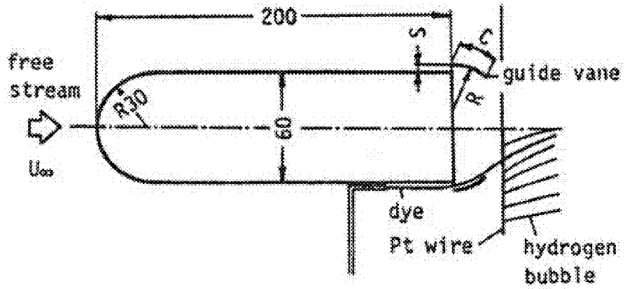
Figure 15: Kato Experimental Set-up
