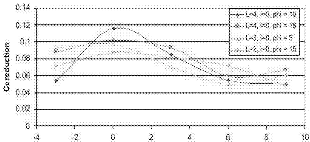
Figure 18: Maragno's Yaw Angle Results
