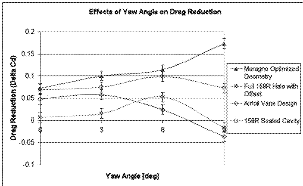
Figure 29: Final Yaw Angle Investigation Results
