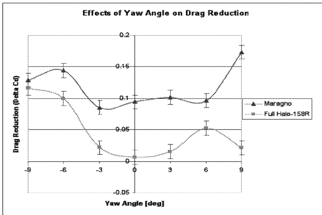
Figure 30: Initial Yaw Angle Study Results
