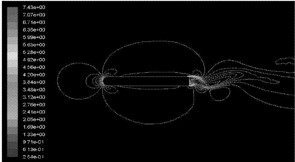
Figure 5: Bluff Body Flow Field in Oscillating Wake
