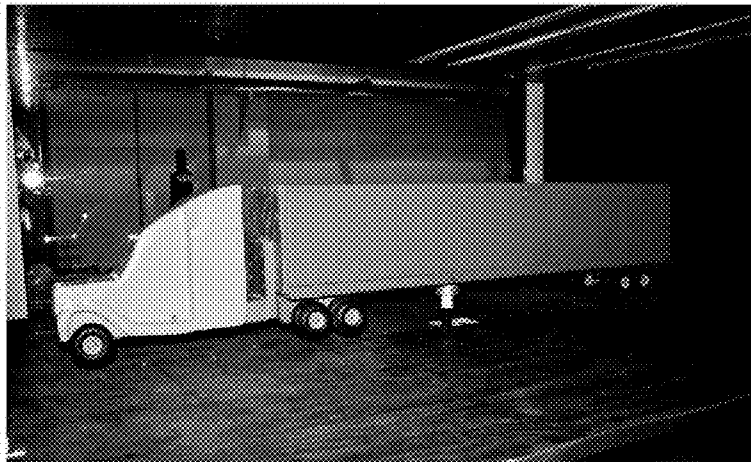
Figure 6: Tractor trailer model in wind tunnel
