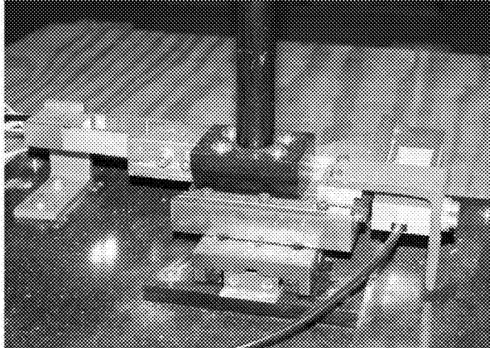
Figure 8: Force Balance Set-up
