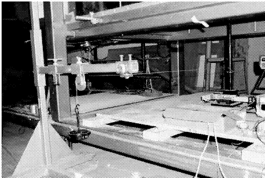
Figure 10: Calibration device
