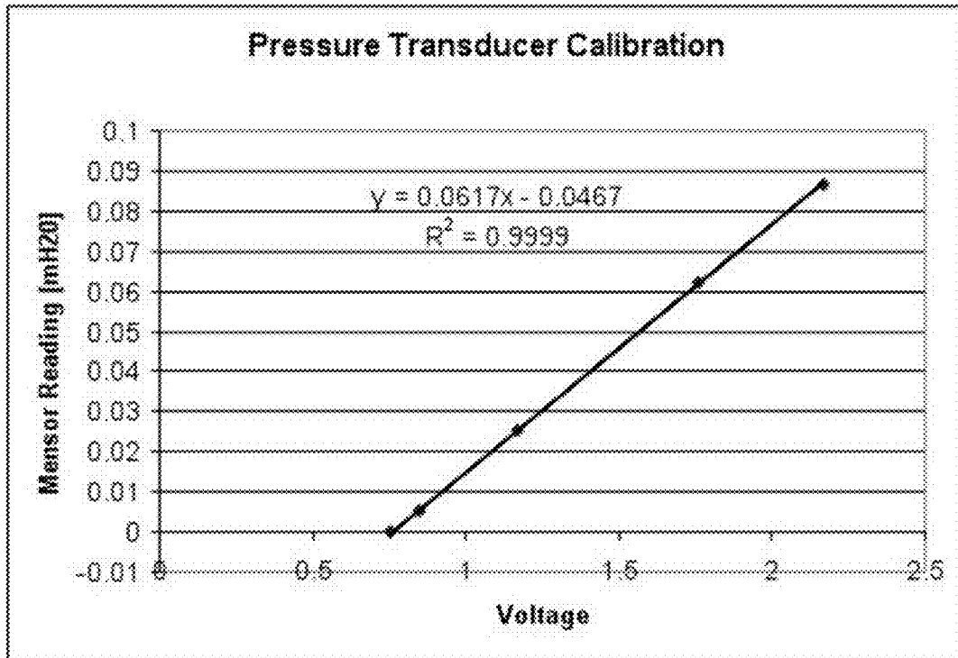
Figure 11: Sample Calibration Curve
