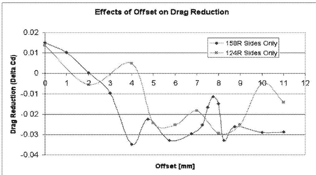
Figure 28: Offset Effects on Drag Reduction
