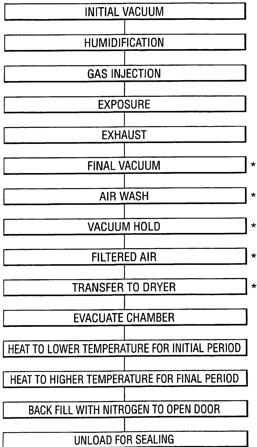
FIG. 1 (PRESENT INVENTION)
