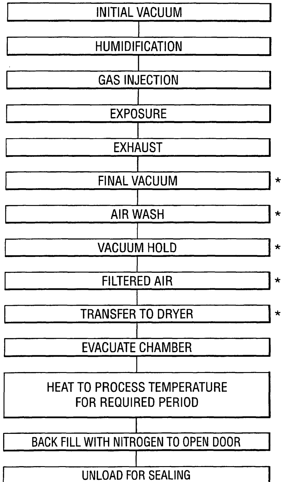
FIG. 2 (CONVENTIONAL PROCESS)
