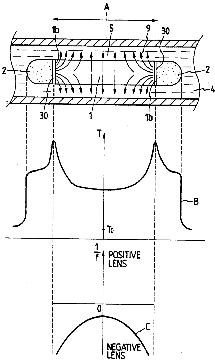
FIG. 3 PRIOR ART
