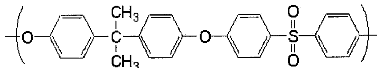
[Chem. 4]
