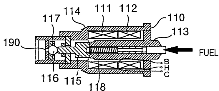
FIG.21A DRAWING OF INJECTOR STRUCTURE
