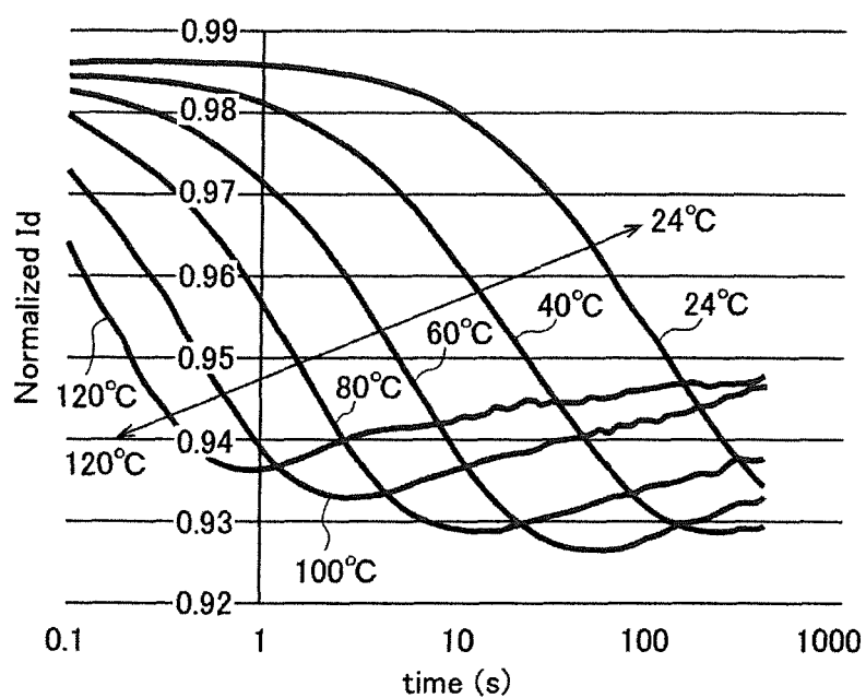
CHANGE IN NORMALIZED ID OVER TIME
