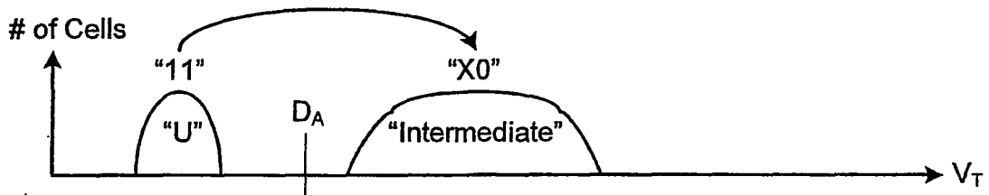
Lower Page Programming (LM Gray Code)
