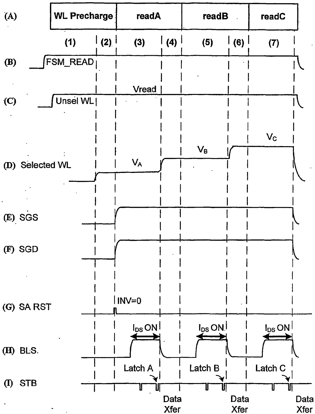
A-B-C READ WITH WORDLINE PRECHARGE
