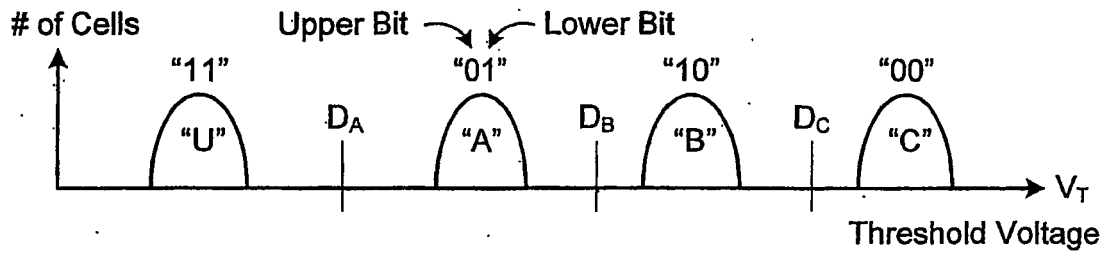
Multistate Memory (LM New Code)
