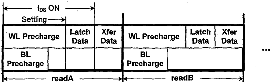
CONVENTIONAL PRECHARGE TIMING FOR SENSING
