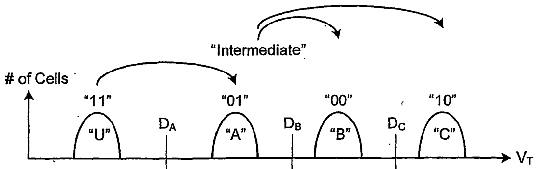
Upper Page Programming (LM Gray Code)
