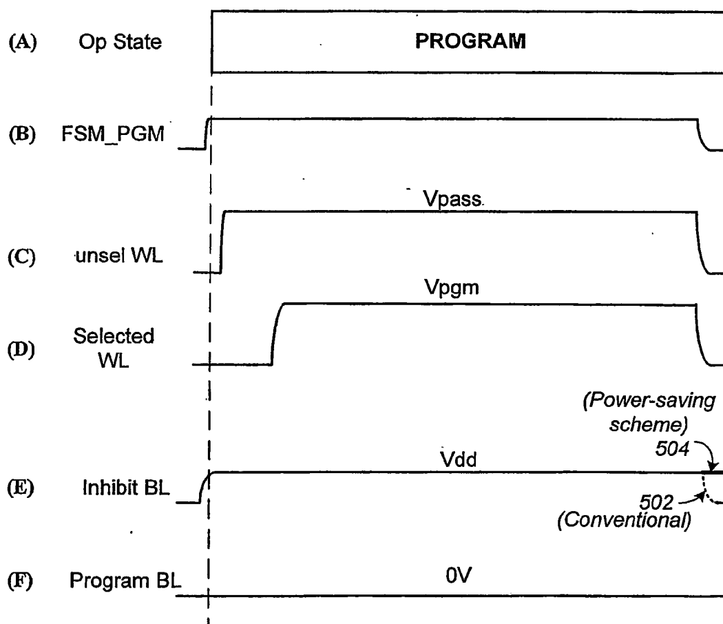
PROGRAM CYCLE TIMING
