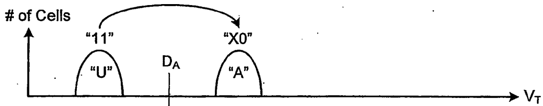
Lower Page Programming (Conventional Gray Code)
