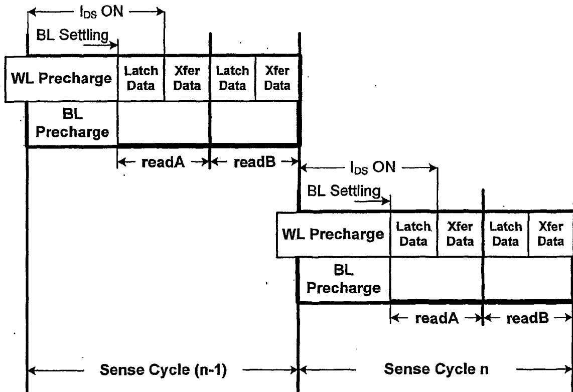
JUMP-START WL PRECHARGE TIMING FOR SENSING
