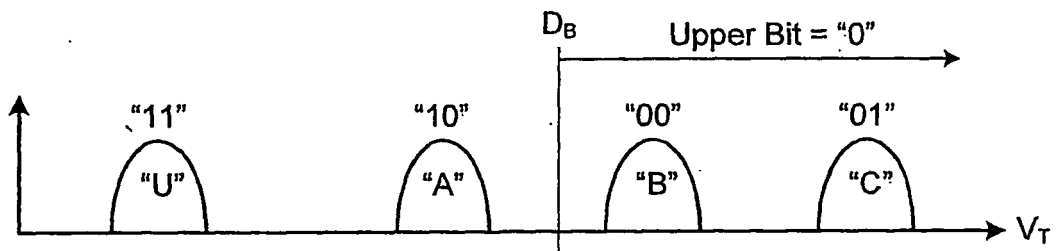
Upper Page Read (Conventional Gray Code)
