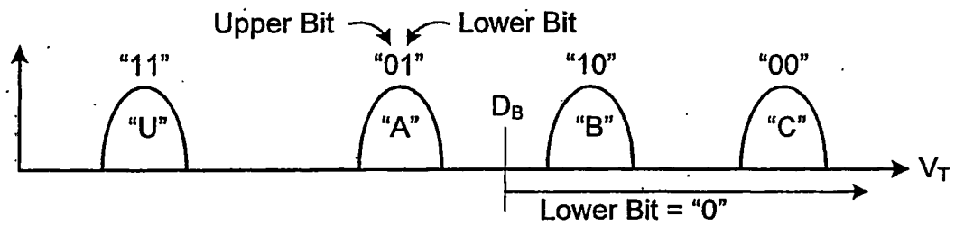
Lower Page Read (LM New Code)
