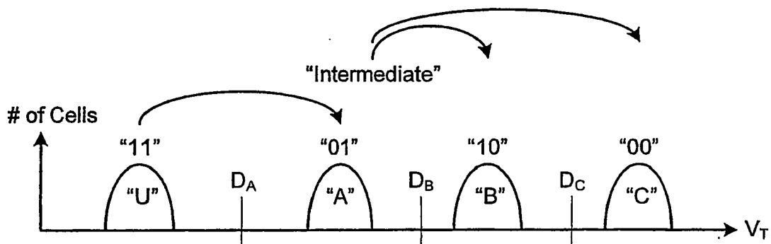
Upper Page Programming (LM New Code)
