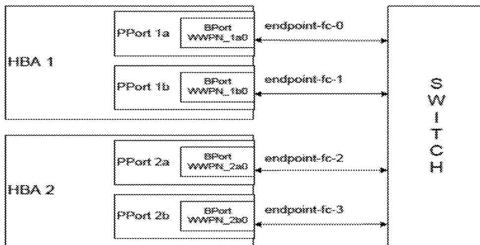
Ports Layout BEFORE Failover is Enabled 702
