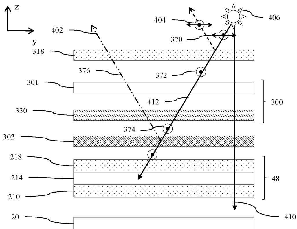
FIG. 17A Reflectivity
