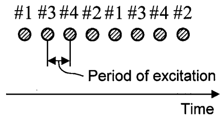
Fig. 4A Without Decompression Device
