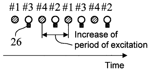
Fig. 4B First Embodiment (Decompression Operating State)
