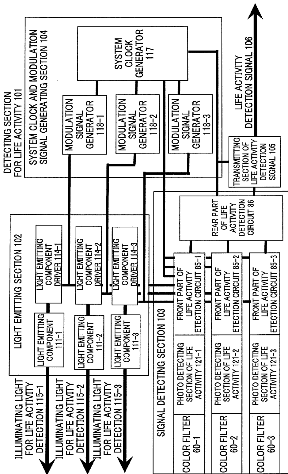
FIG.32 CONFIGURATION OF ANOTHER EXEMPLARY EMBODIMENT OF DETECTING SECTION FOR LIFE ACTIVITY
