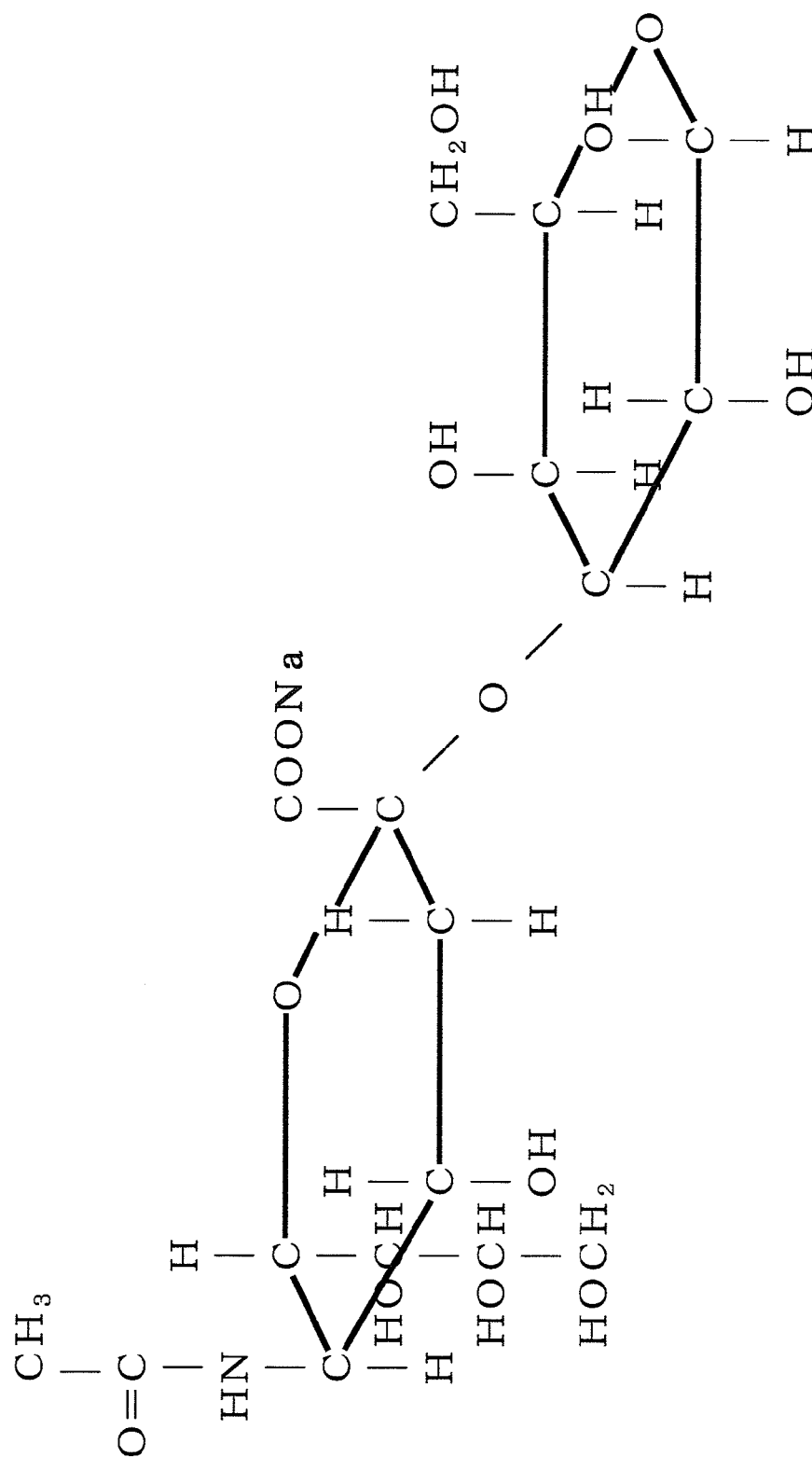
FIG. 7 Part of GD1a structure used for calculating infrared spectral characteristics
