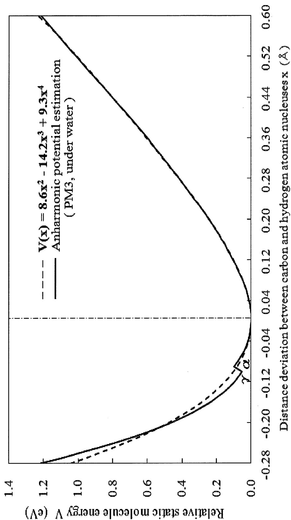
FIG.11 Relative static molecule energy vs. distance deviation between carbon and hydrogen atomic nuclei.
