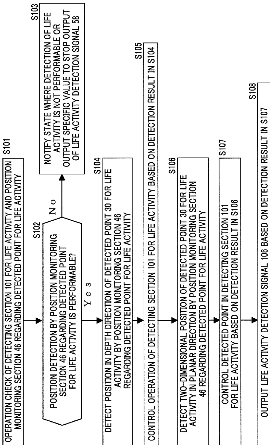
FIG.64 EXPLANATORY VIEW OF A MEASURING METHOD 1 OF LIFE ACTIVITY IN THE APPLIED EMBODIMENT
