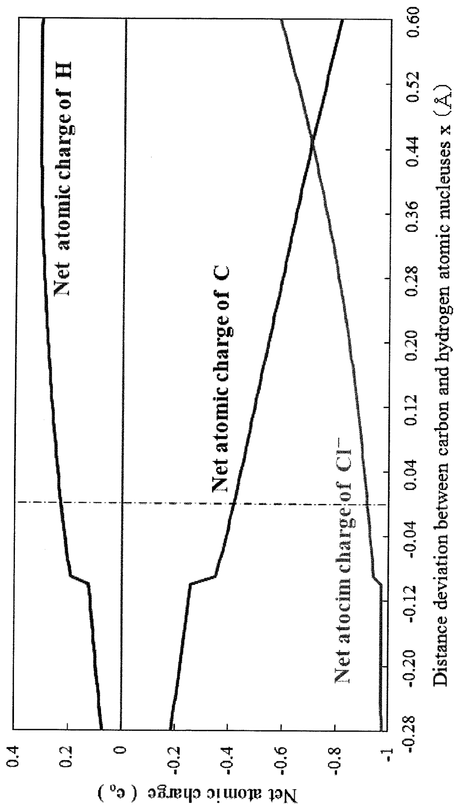
FIG. 14 Net atomic charges vs. distance deviations between carbon and hydrogen atomic nuclei
