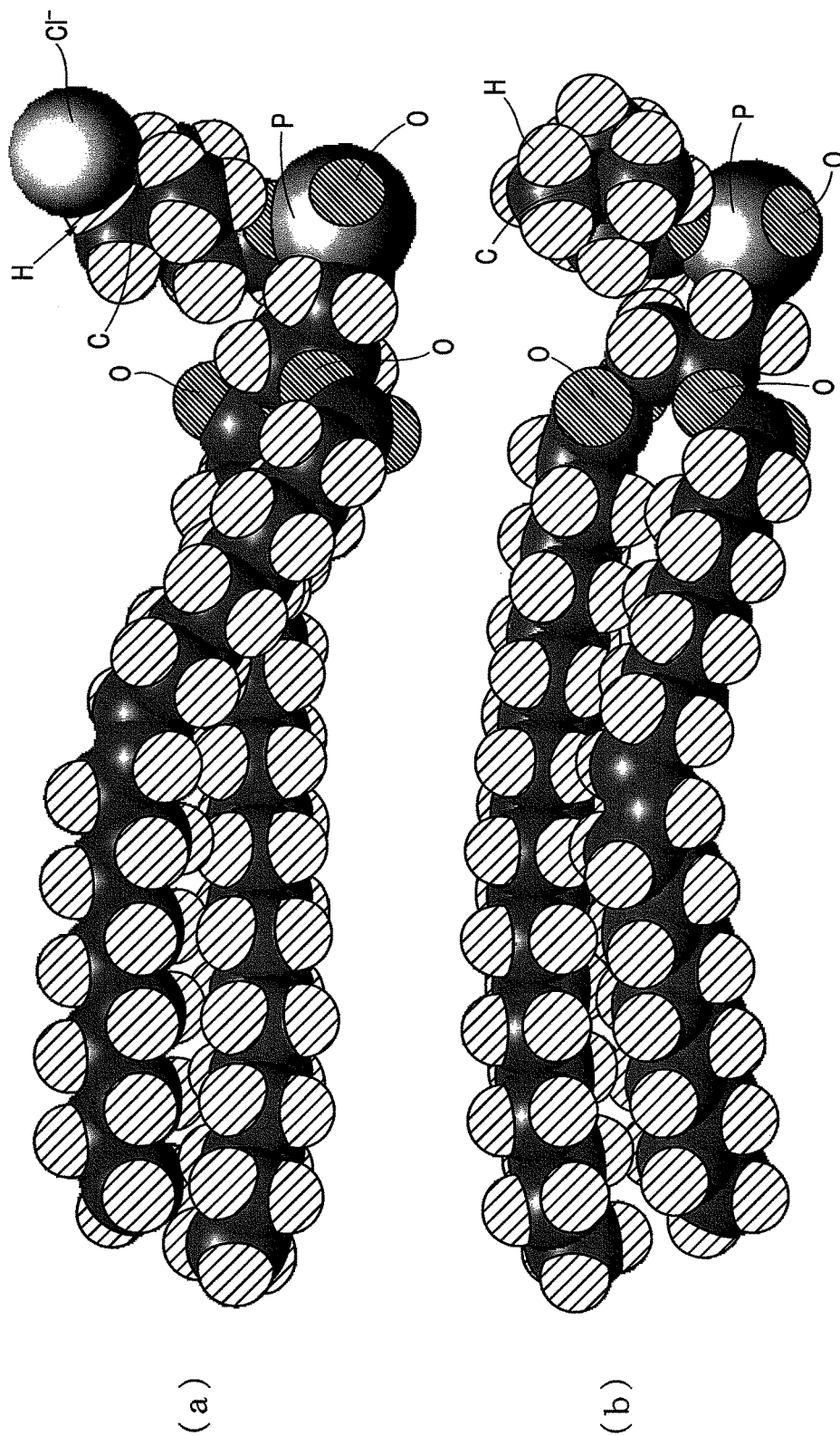
FIG. 5 Estimated molecular structure of PCLN in case of \text{Cl}^- ion attachment and detachment
