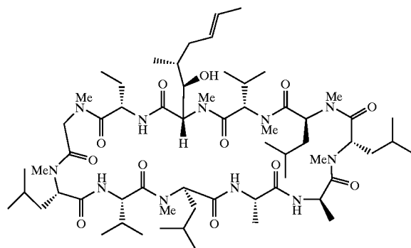
Cyclosporin A
