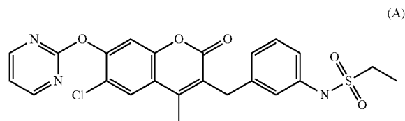
[Chemical Formula 178]
