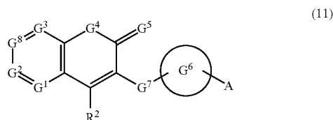
[Chemical Formula 1]
