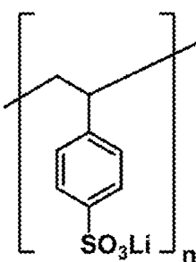
Poly(lithium-4-styrenesulfonate)
