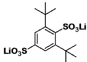
lithium 2,6-di- tert -butylbenzene-1,4-disulfonate
