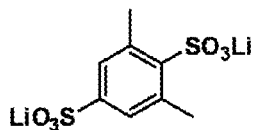
lithium 2,6-dimethylbenzene-1,4-disulfonate
