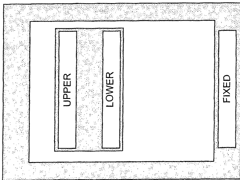
CROSS-SECTION SHOWING MEMS BEAM (UPPER AND LOWER ELECTRODES WITH \text{SiO}_2 BETWEEN THEM, ON SIDES, AND OVER/UNDER)
