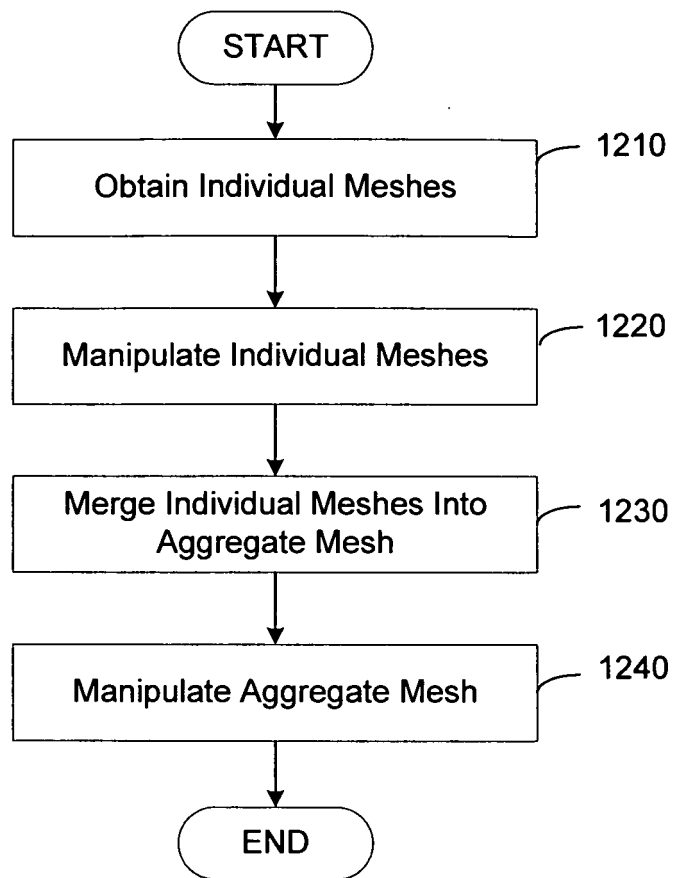
FIG. 12 Mesh Generation
