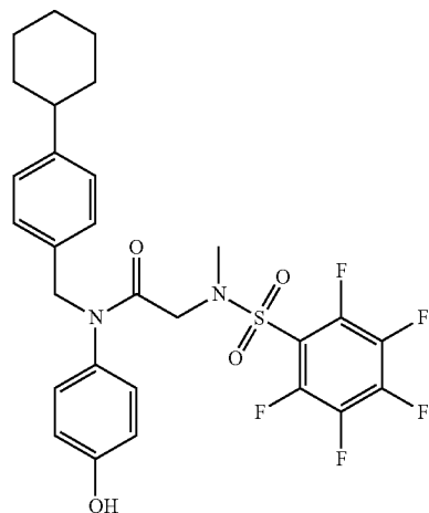
N-(4-cyclohexylbenzyl)-N-(4-hydroxyphenyl)-2-(2,3,4,5,6-pentafluoro-N-methylphenylsulfonamido)acetamide
