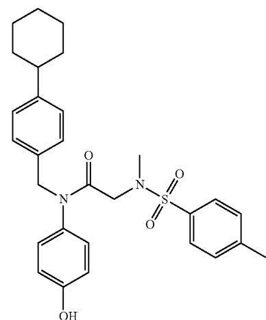
N-(4-cyclohexylbenzyl)-2-(N,4-dimethylphenylsulfonamido)-N-(4-hydroxyphenyl)acetamide
