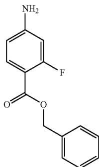
benzyl 4-amino-2-fluorobenzoate
