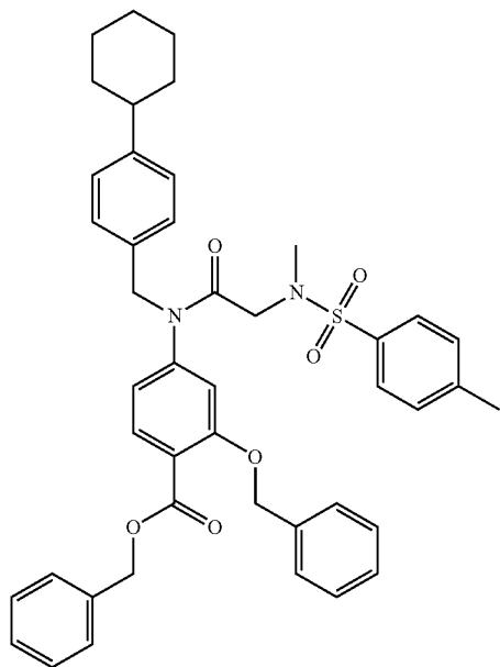
benzyl 2-(benzyloxy)-4-(N-(4-cyclohexylbenzyl)-2-(N,4-dimethylphenylsulfonamido)acetamido)benzoate
