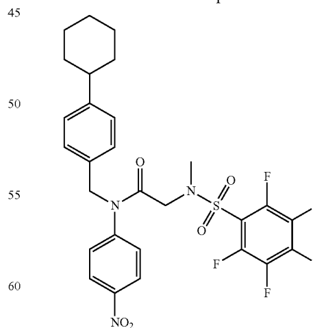
N-(4-cyclohexylbenzyl)-N-(4-nitrophenyl)-2-(2,3,4,5,6-pentafluoro-N-methylphenylsulfonamido)acetamide
