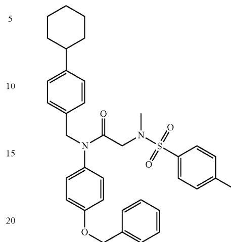
N-(4-(benzyloxy)phenyl)-N-(4-cyclohexylbenzyl)-2-(N,4-dimethylphenylsulfonamido)acetamide
