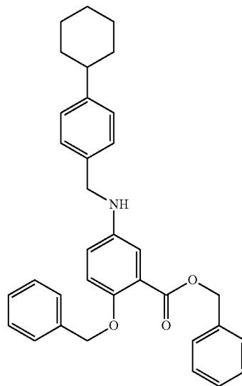
benzyl 2-(benzyloxy)-5-((4-cyclohexylbenzyl)amino)benzoate
