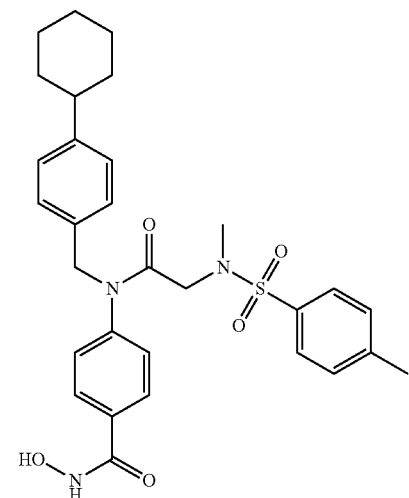
4-(N-(4-cyclohexylbenzyl)-2-(N,4-dimethylphenylsulfonamido)acetamido)-N-hydroxybenzamide
