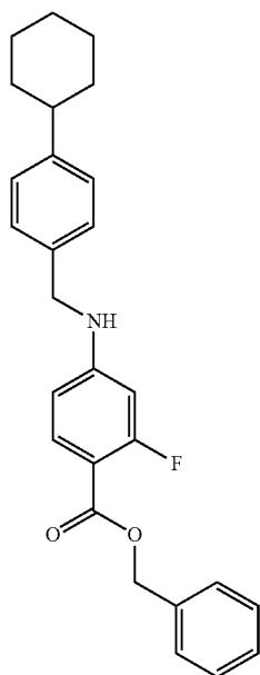
benzyl 4-((4-cyclohexylbenzyl)amino)-2-fluorobenzoate
