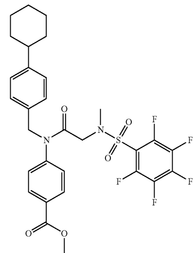
methyl 4-(N-(4-cyclohexylbenzyl)-2-(2,3,4,5,6-pentafluoro-N-methylphenylsulfonamido)acetamido)benzoate
