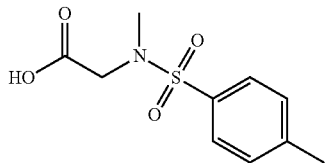
2-(N,4-dimethylphenylsulfonamido)acetic acid
