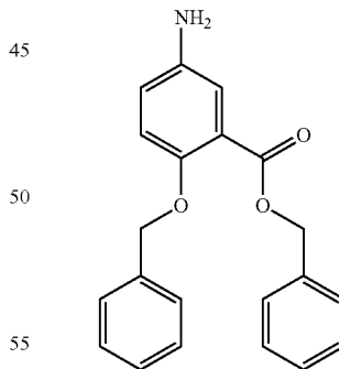
benzyl 5-amino-2-(benzyloxy)benzoate
