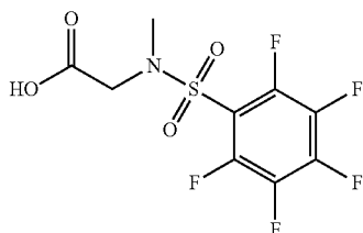
2-(2,3,4,5,6-pentafluoro-N-methylphenylsulfonamido)acetic acid
