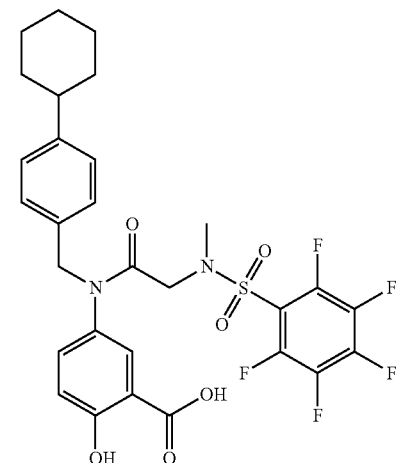
5-(N-(4-cyclohexylbenzyl)-2-(2,3,4,5,6-pentafluoro-N-methylphenylsulfonamido)acetamido)-2-hydroxybenzoic acid
