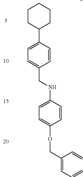
4-(benzyloxy)-N-(4-cyclohexylbenzyl)aniline
