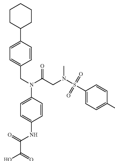
2-((4-(N-(4-cyclohexylbenzyl)-2-(N,4-dimethylphenylsulfonamido)acetamido)phenyl)amino)-2-oxoacetic acid
