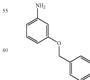
3-(benzyloxy)aniline
