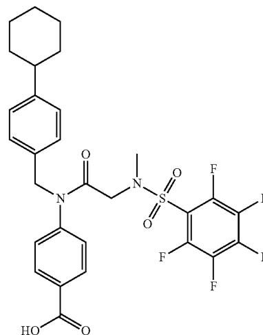
4-(N-(4-cyclohexylbenzyl)-2-(2,3,4,5,6-pentafluoro-N-methylphenylsulfonamido)acetamido)benzoic acid
