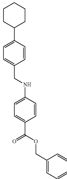
benzyl 4-((4-cyclohexylbenzyl)amino)benzoate
