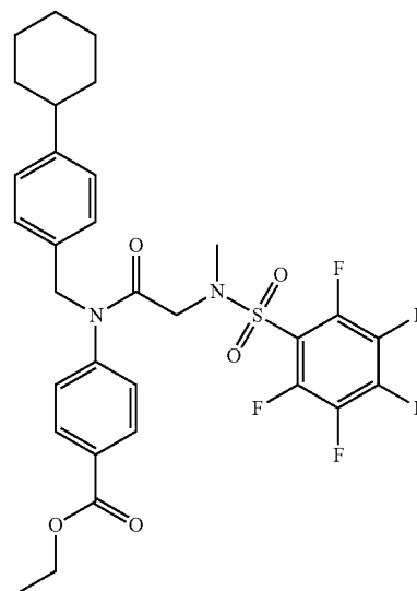
ethyl 4-(N-(4-cyclohexylbenzyl)-2-(2,3,4,5,6-pentafluoro-N-methylphenylsulfonamido)acetamido)benzoate
