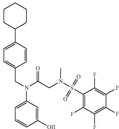
N-(4-cyclohexylbenzyl)-N-(3-hydroxyphenyl)-2-(2,3,4,5,6-pentafluoro-N-methylphenylsulfonamido)acetamide
