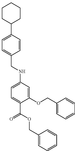
benzyl 2-(benzyloxy)-4-((4-cyclohexylbenzyl)amino)benzoate
